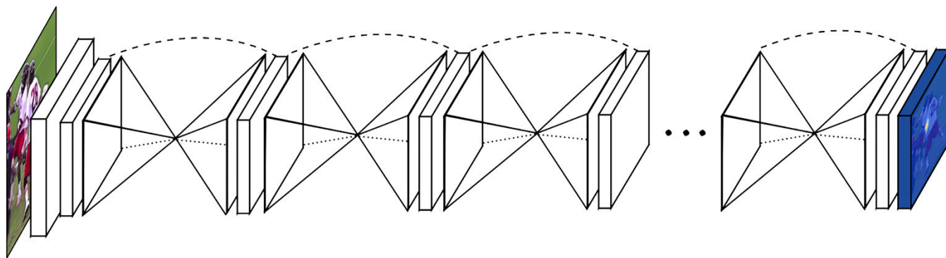
FIGURE 12. The overall structure of stacked hourglass modules.
