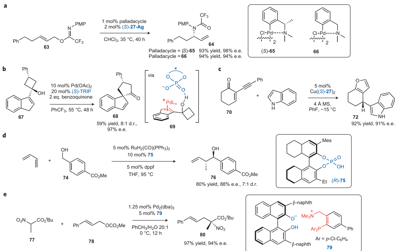
Figure 7 | Further examples of asymmetric metal catalysis with chiral counterions. a , Overman rearrangement using a cationic palladium complex with a chiral phosphate anion. b , Semi-Pinacol rearrangement initiated by allylic C–H activation and proceeding through a cationic palladium intermediate paired with a chiral phosphate anion. c , Copper-catalysed cycloisomerization/addition reaction in which a chiral phosphate is responsible for the observed enantioselectivity. d , Ruthenium catalysis in combination with chiral phosphates for the hydrohydroxyalkylation of butadiene. e , Allylic alkylation of \alpha -nitrocarboxylates using catalyst 79 in which a chiral binaphtholate is ion-paired with a quaternary ammonium salt incorporated into a phosphine ligand. PMP, para -methoxyphenyl; Mes, 1,3,5-trimethylphenyl; dppf, 1,1'-bis(diphenylphosphino)ferrocene; dba, dibenzylideneacetone; d.r., diastereometric ratio.
