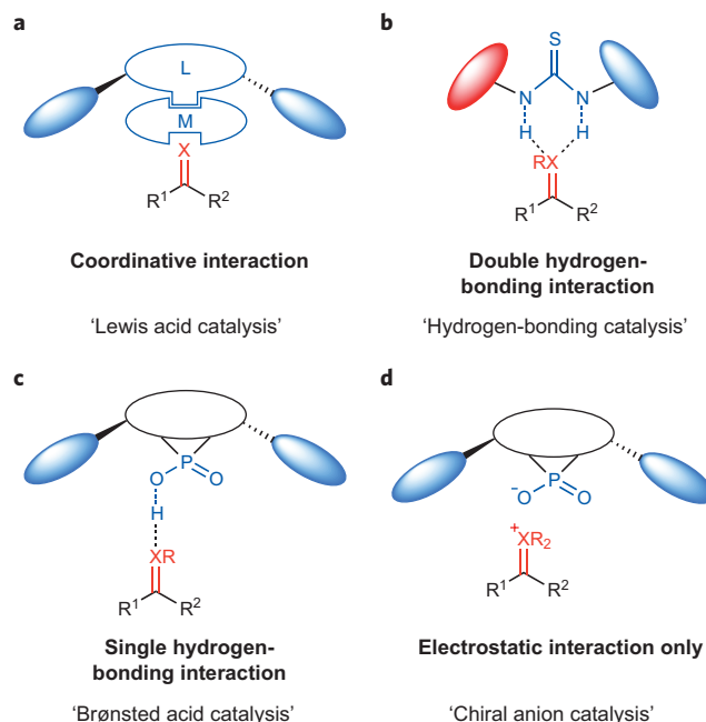
Figure 1 | Representative asymmetric activation modes of a carbonyl group or imine. M, metal; L, ligand.
