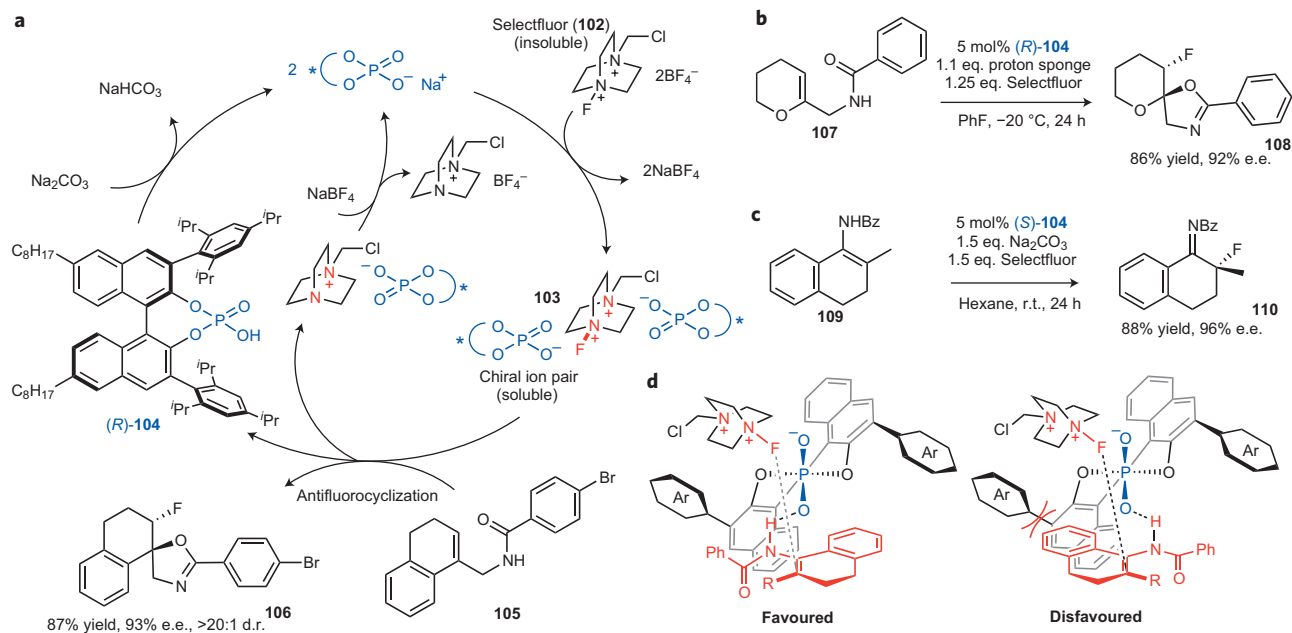
Figure 9 | Examples of the use of chiral anions in asymmetric phase-transfer catalysis. a , Proposed catalytic cycle for the fluorocyclization of dihydronaphthalene derivatives showing the proposed chiral Selectfluor species after double anion exchange ( 103 ). b , Fluorocyclization of an enol ether using this concept. c , Fluorination of enamides using chiral anion phase-transfer catalysis. d , Proposed model to rationalize the absolute stereochemistry observed in the latter transformation. Bz, benzoyl.
