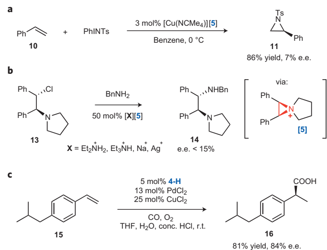
Figure 3 | Early efforts towards asymmetric catalysis using chiral anions. a , Chiral borate anions provide some enantioselectivity in a copper-catalysed aziridination. b , Efforts towards asymmetric ring opening of prochiral aziridinium ions using the same chiral borate anion. c , Hydrocarboxylation of a styrene using a chiral phosphoric acid in combination with palladium and copper catalysis. Ts, para -toluenesulfonyl; Bn, benzyl; THF, tetrahydrofuran; r.t., room temperature.
