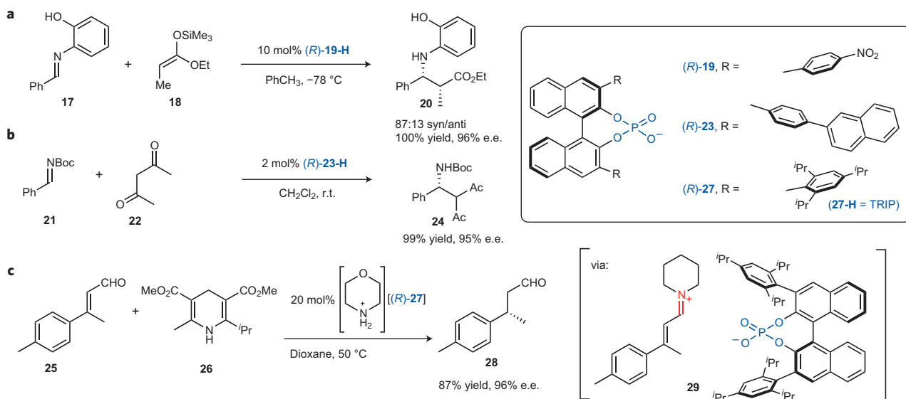
Figure 4 | Some seminal applications of 3,3'-disubstituted BINOL-derived phosphoric acids. a , Asymmetric addition of silyl enol ethers to imines via Brønsted acid catalysis. b , Asymmetric addition of acetylacetone to imines by Brønsted acid catalysis. c , Asymmetric reduction of enals through chiral anion catalysis. i Pr, iso -propyl; Boc, tert -butoxycarbonyl.
