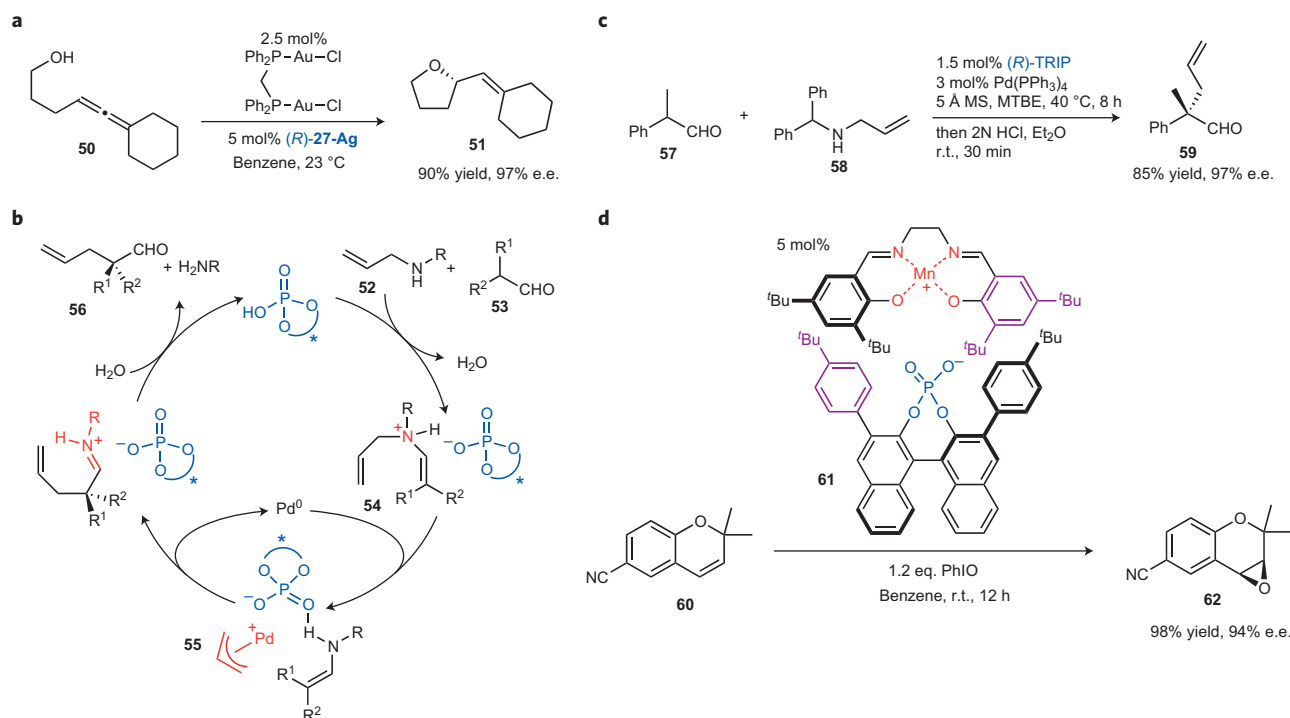
Figure 6 | Examples of asymmetric metal catalysis with chiral anionic counterions. a , Hydroalkoxylation of allenes using a gold catalyst with a chiral phosphate anion. b , Mechanistic hypothesis for Tsuji-Trost reaction using a palladium catalyst with chiral phosphate anion. c , Successful example of the latter reaction. d , Epoxidation of alkenes using a catalyst derived from a cationic achiral Mn-salen complex and a chiral phosphate anion.
