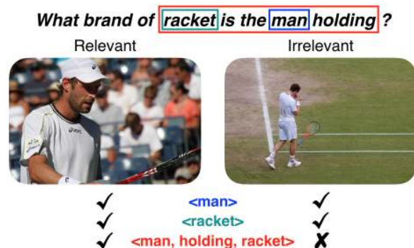
Figure 1: Questions asked about images often contain ‘premises’ that imply visual semantics. From the above question, we can infer that a relevant image must contain a man, a racket, and that the man must be holding the racket. We extract these premises from visually grounded questions and use them to construct a new dataset and models for question relevance prediction. We also find that augmenting standard VQA training with simple premise-based questions results in improvements on tasks requiring compositional reasoning.
