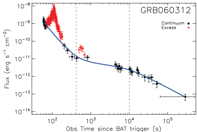
Figure 2. 0.3-10 keV unabsorbed flux LC of GRB 060312 with best-fitting model superimposed (blue solid line). The red crosses mark the data points identified as “excesses” during the semi-automatic fitting routine and subsequently removed from the fit to obtain the best-fitting power-law plus broken power-law model. Vertical dashed lines: best estimates of the break times obtained as described in the main text.
