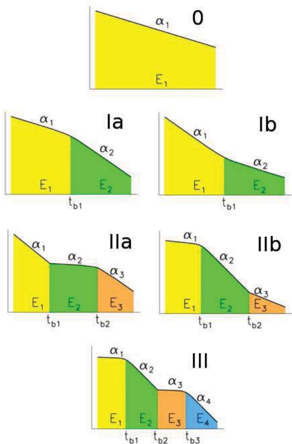
Figure 1. Cartoon showing the different LC models used in this work. Both axes use logarithmic units.
