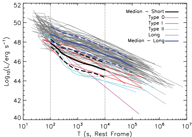
Figure 3. Best fitting profiles of 9 C-like short GRBs with rest-frame time coverage 10^2 - 10^4 s (colour lines) superimposed on the sample of long GRBs (grey lines). Black (blue) solid line: median \text{Log}(L) light-curve for short (long) GRBs; dashed lines mark the 1\sigma dispersion. The LCs have been calibrated in the rest-frame 0.3-30 keV energy band.
