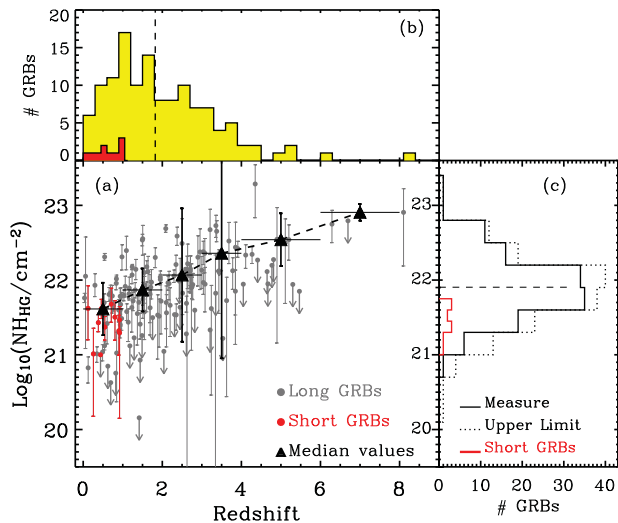
Figure 5. Left panel: (a): Intrinsic neutral hydrogen absorption vs. redshift for long and short GRBs (grey and red dots, respectively). 90% upper limits are marked with arrows. Median \text{NH}_{\text{HG}} values in different redshift bins are indicated with filled triangles: for each bin, the error bars span the 1\sigma \text{NH}_{\text{HG}} dispersion. (b): redshift distribution of the sample of long (yellow) and short (red) GRBs. (c): Intrinsic neutral hydrogen distribution for long (black line) and short (red line) GRBs. The dashed histogram includes upper limits. In panels (b) and (c) a dashed line indicates the median value for the entire distributions ( \langle z \rangle = 1.82 , \langle \text{NH}_{\text{HG}} \rangle = 10^{21.8} \text{ cm}^{-2} ).
