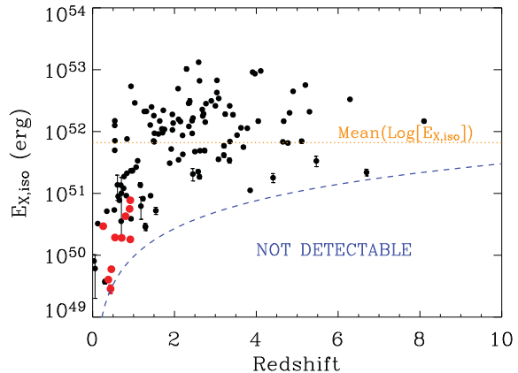
Figure 4. 0.3-30 keV (rest-frame) X-ray energy as a function of redshift. Black (red) points: long (short) GRBs. Blue dashed line: empirically derived detectability threshold. For z > 2 we are not sensitive to GRBs with E_{X,\text{iso}} \lesssim 10^{51} erg. For z > 1 there is no evidence for an evolution of the upper bound of E_{X,\text{iso}} with redshift.
