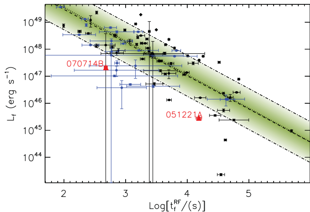
Figure 7. Luminosity at the end of the plateau phase, 0.3-30 keV (rest-frame) vs. end-time of the plateau. Colour coding as in Fig. 6. Blue points are for type Ia LCs.
