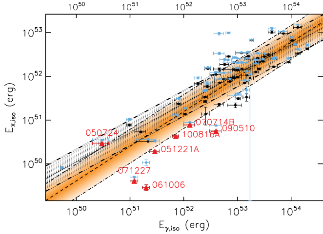
Figure 9. Impact of the temporal extrapolation of the observed LCs on the E_{X,iso} vs. E_{\gamma,iso} correlation. Colour coding as in Fig. 6. Light blue dots: E_{X,iso} values have been computed integrating the luminosity over a common rest-frame interval of time.
