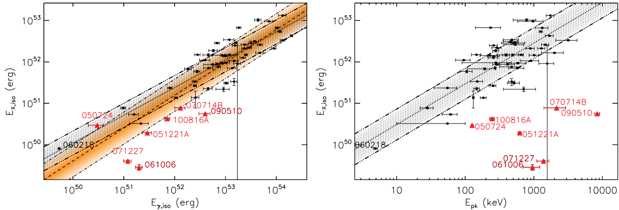
Figure 6. Correlations involving E_{\gamma,\text{iso}} ( 1 - 10^4 keV, rest-frame), E_{X,\text{iso}} (0.3-30 keV, rest-frame) and the rest-frame prompt peak energy E_{\text{pk}} . Black dots (red triangles): long (short) GRBs. Dashed line: best-fitting power-law model for the entire short plus long GRBs sample. Dotted line: best-fitting model for the long GRB class, only. The coloured and hatched areas mark the 68% confidence region around the best fit. Short GRBs and outliers are named.
