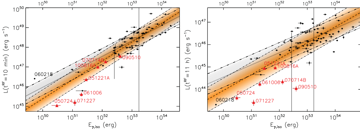
Figure 8. 0.3-30 keV (rest-frame) X-ray LC luminosity measured at 10 minutes (left panel) and 11hr (right panel) rest-frame vs. E_{\gamma,\text{iso}} . Colour coding as in Fig. 6. The scatter of the correlation increases with time.
