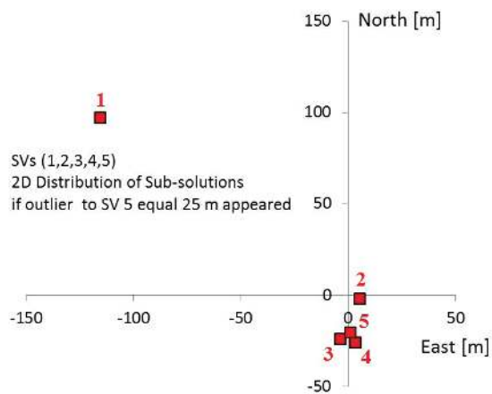
Fig. 13. Distribution of sub-solutions if outlier equal 25 m appeared in pseudorange measurement to SV5. Red squares marked shift of sub-solutions related to the positioning solution. Numbers at squares indicate number of satellite excluded from the positioning solution
