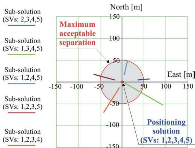
Fig. 6. Obtained sub-solutions distribution related to the positioning solution if outlier equal 100 m appeared in pseudorange measurements to SV1
