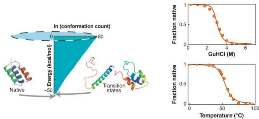
Figure 7. (Left) The density of states (DOS) cartoonized as an energy landscape for the three-helix bundle protein F13W*: DOS (x-axis) versus the energy (y-axis). (Right) Denaturation predictions versus experiments (146). The peak free energy (here, where the DOS is minimum), typically taken to be the transition state, is energetically very close to native.
