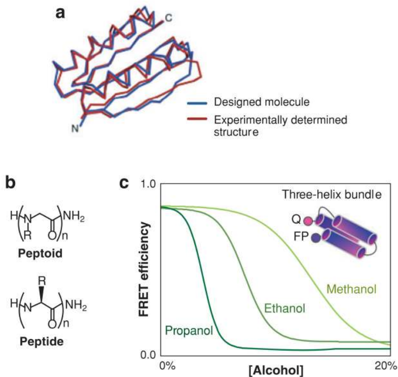
Figure 2. (a) A novel protein fold, called Top7, designed by Kuhlman et al. (129). Designed molecule ( blue ) and the experimental structure determined subsequently ( red ). From Reference 129; reprinted with permission from AAAS. (b) Three-helix bundle foldamers have been made using nonbiological backbones (peptoids, i.e., N-substituted glycines). (c) Their denaturation by alcohols indicates they have hydrophobic cores characteristic of a folded molecule (134).
