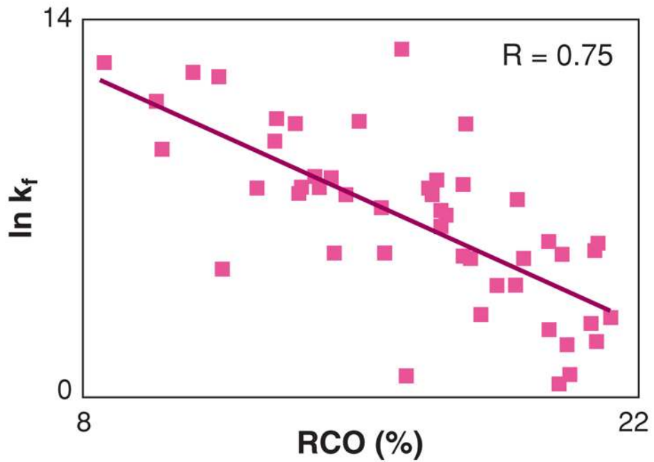
Figure 4. Folding rate versus relative contact order (a measure of localness of contacts in the native structure) for the 48 two-state proteins given in Reference 91, showing that proteins with the most local contacts fold faster than proteins with more nonlocal contacts.
