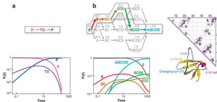
Figure 8. (a) A simple single-pathway system. R, reactant; TS, transition state; P, product. (b) Pathway diagram of SH3 folding from a master-equation model. The native protein has five contact clusters: A = RT loop; B = \beta_2\beta_3 ; C = \beta_3\beta_4 ; D = RT loop- \beta_4 ; and E = \beta_1\beta_5 . Combined letters, such as BD, mean that multiple contact clusters have formed. Funneling occurs toward the right, because the symbols on the left indicate large ensembles, whereas the symbols on the right are smaller ensembles. The numbers indicate free energies relative to the denatured state. The arrows between the states are colored to indicate transition times between states. The slowest steps are in red; the fastest steps in green. BD is the transition state ensemble because it is the highest free energy along the dominant route. While B and BD would seem to be obligatorily in series, the time evolutions of these states show that they actually rise and fall in parallel (232).
