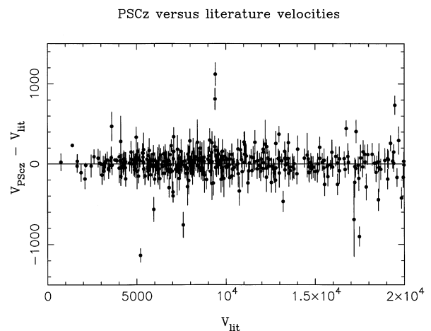
Figure 3. PSC z versus literature redshifts. Error bars show combined errors.
