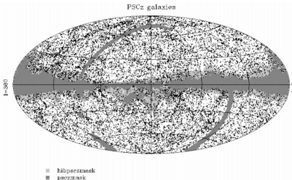
Figure 1. 15 431 PSC z sources identified as possible or definite galaxies, high l and default masks in galactic coordinates.
