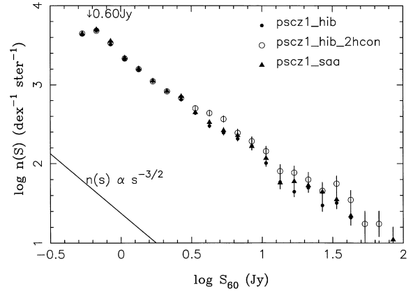
Figure 7. Source counts for all high-latitude sky (filled circles), high-latitude 2-HCON sky (open circles) and an area with potential SAA problems (triangles).
