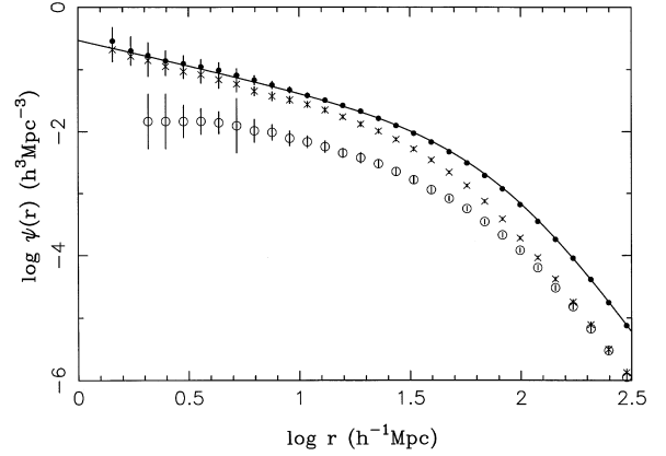
Figure 6. Parametric and non-parametric selection functions for the high-latitude PSCz survey (line and filled circles). Also shown are the QDOT (open circles) and 1.2-Jy (crosses) non-parametric selection functions.
