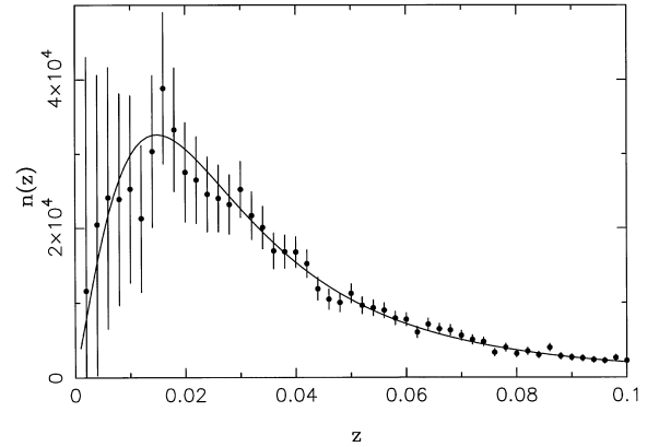
Figure 5. n(z) distribution for the high-latitude PSCz survey. Error bars are J_3 -weighted. The line is the prediction from the selection function.
