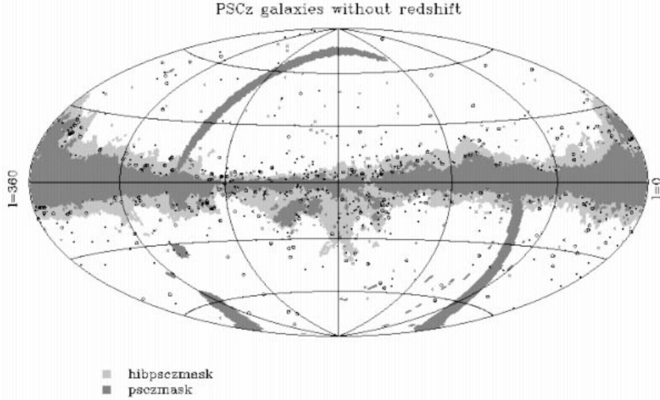
Figure 4. Sky distribution of PSCz sources without redshift, with galaxy identifications b_J < 19.5 mag (open circles, 192 sources) and fainter than this or with no identification (crosses, 542 sources).
