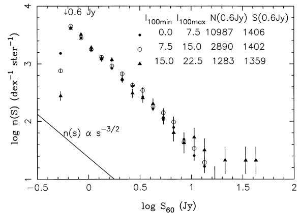
Figure 8. Source counts for identified PSCz galaxies as a function of 100- \mu\text{m} background, I_{100} < 7.5 \text{ MJy sr}^{-1} (filled circles), 7.5–15 (open circles) and 15–22.5 (triangles).
