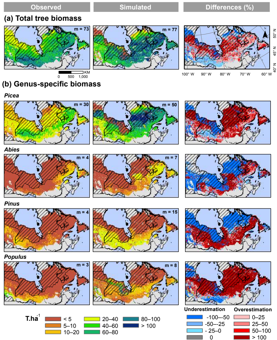
Figure 4. (a) Observed, LPJ-LMfire simulated, and differences (%) in mean total aboveground biomass ( T ha^{-1} ) between 2000 and 2006 across eastern boreal Canada. (b) Genus-specific aboveground biomass. The observed aboveground biomass maps across Canada were predicted and validated with photo-plot information in the southern areas (non-hatched areas) and data published by Beaudoin et al. (2014). Median ( m ) tree aboveground biomass values are also indicated for each map; these were calculated for the non-hatched areas at a 10 km resolution.
