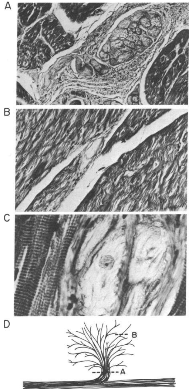
FIGURE 8 Purkinje fiber innervation of the left ventricular free wall in the porcine heart. (a) Subendocardial bundle of Purkinje fibers surrounded by thick connective tissue sheath (GTAF, \times 250 ). (b) Two Purkinje fibers located in the subepicardium (GTAF, \times 250 ). (c) Purkinje fibers and neighboring cardiac muscle. Cytoplasm is generally clear containing only prominent nucleus and scattered fibrillar material (GTAF, \times 1,000 ). (d) Model of Purkinje fiber innervation in the left ventricular free wall. The concentration of the fibers is greatest in the subendocardial layers gradually thinning and branching out as the epicardial surface is approached.
