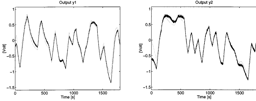
Fig. 3. Validation of the minimum-phase model G_- . The outputs from the model (dashed lines) together with the outputs from the real process (solid lines) are shown.
