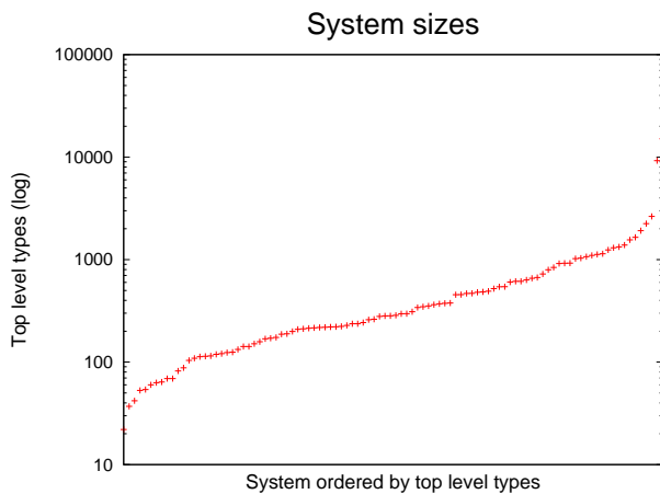
Figure 3. Distribution of sizes of systems.
