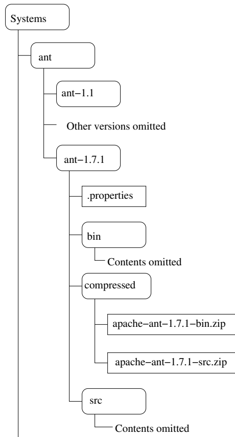
Figure 1. Organisation of Qualitas Corpus.
