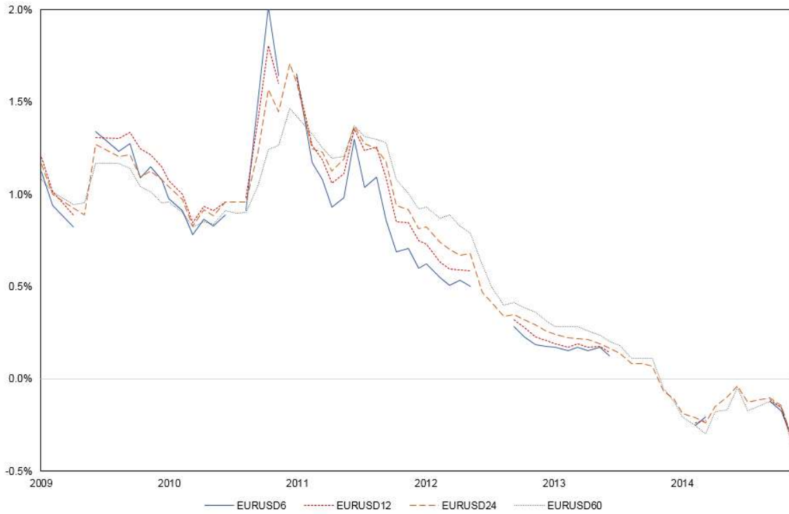
Figure IA.7: Term structure of the euro-dollar risk premium, as measured by QRP, in the time series for horizons of 6, 12, 24, and 60 months.
