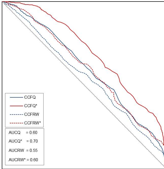
Figure IA.1: Correct classification frontier (CCF) and AUC statistics for the quanto excess return forecast, and a competitor excess return forecast under which exchange rates follow a random walk.
