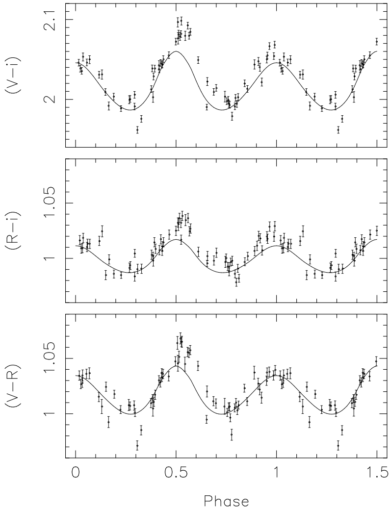
Fig. 8. Photometric data as presented in Fig. 3, from which six data points have been removed (see text). The drawn lines represent a theoretical color curve computed for a binary inclination and secondary mass of ( 68^\circ, 75, 2.10 M_\odot ), an intrinsic luminosity of 41 L_\odot and a disk with a fractional size of 0.80, a flaring angle of 2^\circ and a temperature at the outer edge of 100 K.
