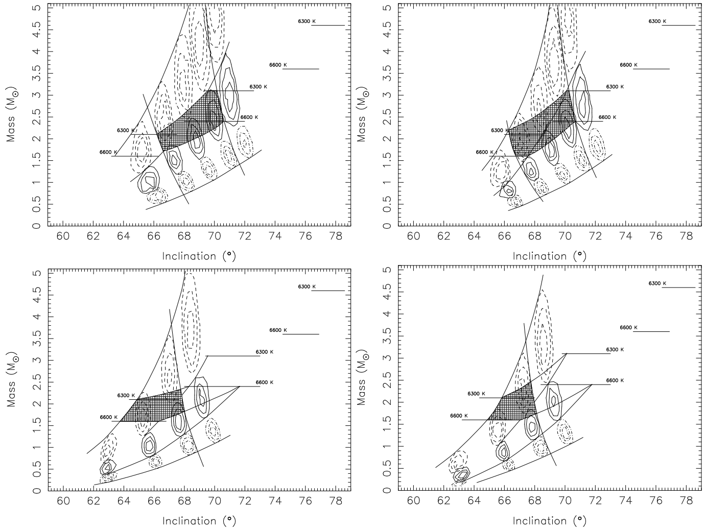
Fig. 6. Total collection of solutions in the i versus M_2 plane for (T_{\text{edge}}, \gamma) = (100 \text{ K}, 2^\circ) [top-left], (1000 \text{ K}, 2^\circ) [top-right], (100 \text{ K}, 10^\circ) [bottom-left], and (1000 \text{ K}, 10^\circ) [bottom-right]. The hatched area's are constructed similar as in Fig. 5.
