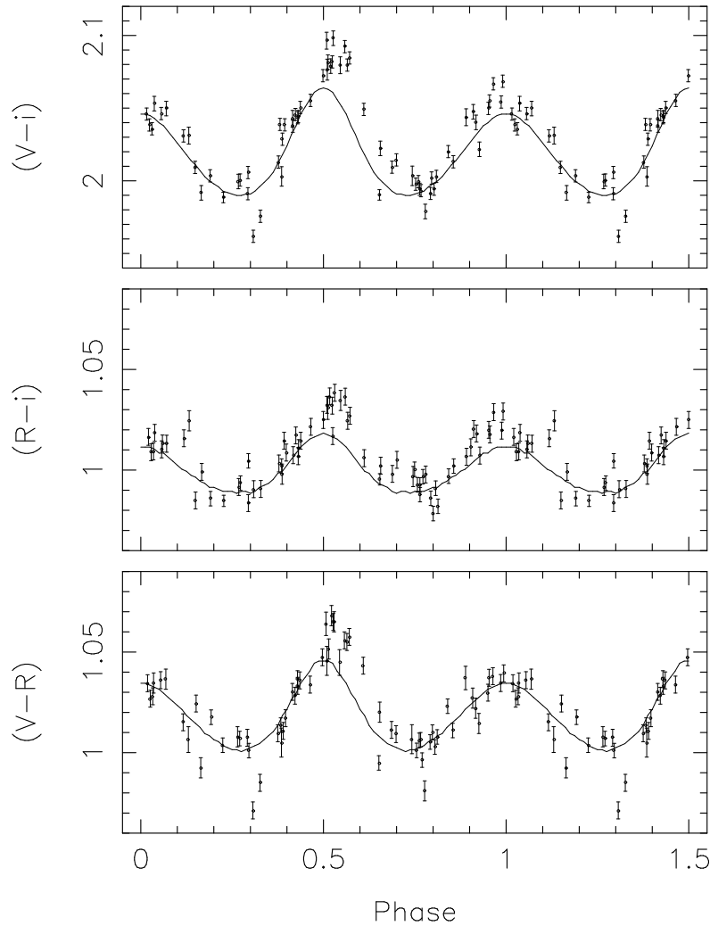
Fig. 3. (V-R) , (R-i) and (V-i) color curves folded at the photometric ephemeris T_{\text{inf}}(\text{HJD}) = 244\,9838.4198(52) + 2.62168(14) \times N . The curves are repeated over 1.5 cycles for clarity. Phase 0.0 corresponds to inferior conjunction of the secondary with respect to the compact star. The drawn lines represent a theoretical color curve computed for a binary inclination and secondary mass of (67^\circ:25, 1.60 M_\odot) .
