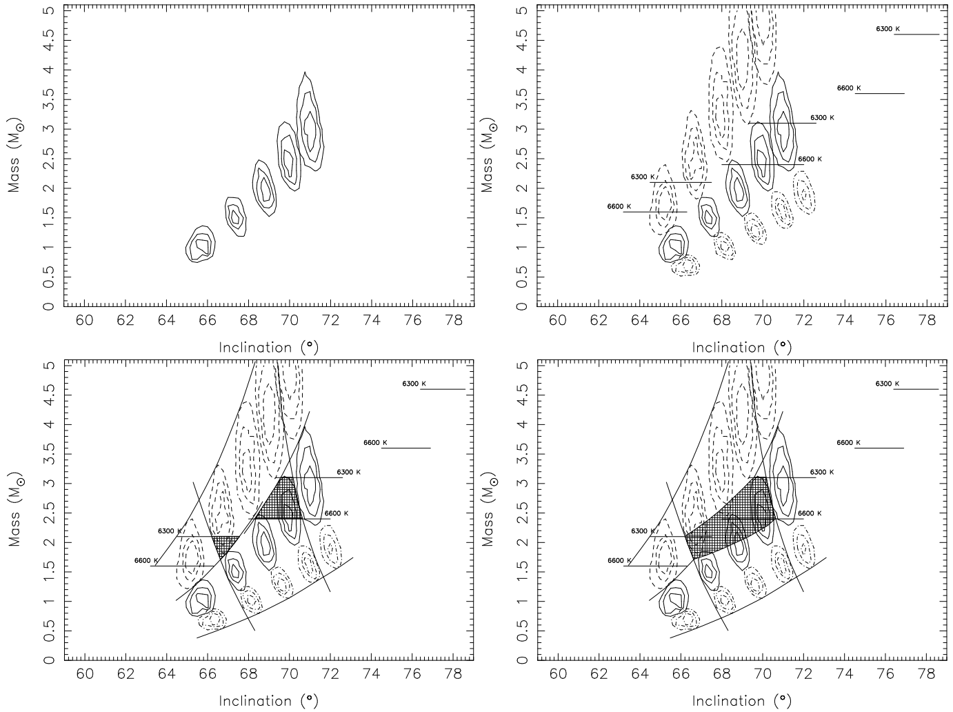
Fig. 5. 1, 2, 3 \sigma confidence contours in the i versus M_2 plane for intrinsic luminosities of 41 [top-left panel], and 31 (dashed), 41 (solid), and 54 L_\odot (dashed-dotted) [other panels], for accretion disk models with outer edge temperature T_{\text{edge}}=100 K, flaring angle \gamma = 2^\circ , and fractional disk radii between 0.6 and 1.0. Average effective temperatures of the secondary star are indicated in the top-right panel. In the bottom-left panel, the solutions are constrained by the smooth curves tangent to the \alpha = 0.7, 0.9 , and 31, 41 and 54 L_\odot confidence contours. The solutions in the i versus M_2 plane which are constrained by these limits are indicated by the hatched area in the bottom-left panel. Finally, the total collection of solutions for this ( T_{\text{edge}}, \gamma ) is given in the bottom-right panel.
