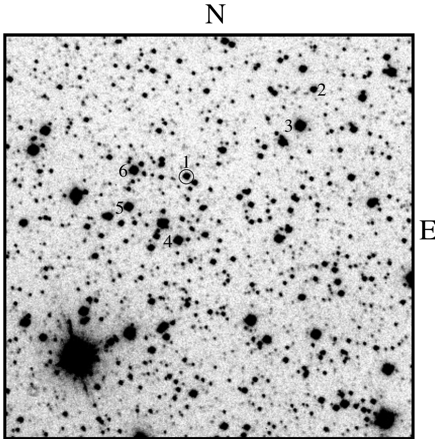
Fig. 1. 3' \times 3' R -band find chart of the field of Nova Sco 1994, taken on 1996 March 5. The exposure time was 300 seconds; North is at the top, East to the right. Nova Sco 1994 is indicated by a circle and is numbered 1, the five comparison stars are numbered 2-6.
