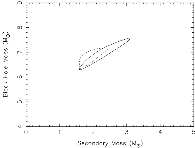
Fig. 9. Collection of solutions in the M_2 versus M_1 plane for a flaring angle of the accretion disk of 2^\circ (solid lines) and 10^\circ (dashed lines). The mass of the secondary star is restricted to 1.6\text{--}3.1 M_\odot , while the mass of the compact object lies in the range 6.29\text{--}7.60 M_\odot .
