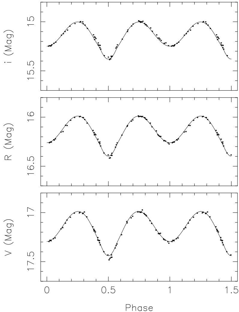
Fig. 7. Photometric data as presented in Fig. 2, from which six data points have been removed (see text). The drawn lines represent a theoretical light curve computed for a binary inclination and secondary mass of ( 68^{\circ}75 , 2.10 M_{\odot} ), an intrinsic luminosity of 41 L_{\odot} and a disk with a fractional size of 0.80, a flaring angle of 2^{\circ} and a temperature at the outer edge of 100 K.
