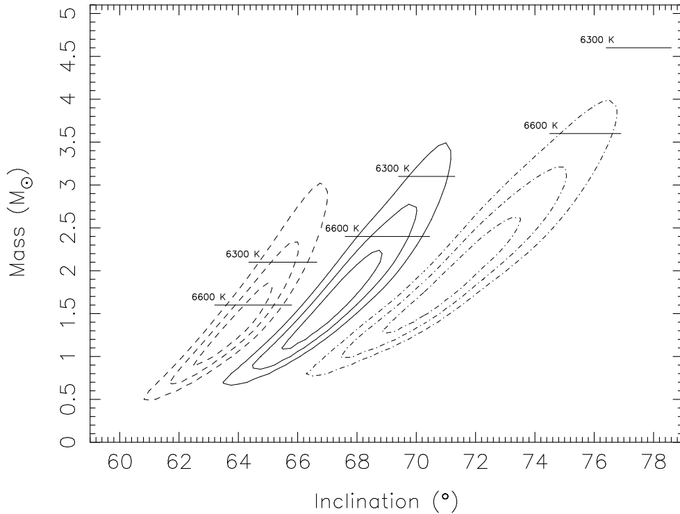
Fig. 4. 1, 2, 3 \sigma confidence contours in the i versus M_2 plane for intrinsic luminosities of 31 (dashed), 41 (solid), and 54 L_\odot (dashed-dotted). The average effective temperatures from the secondary, calculated from the intrinsic luminosity and the effective radius of the secondary, are indicated for 6300 and 6600 K.
