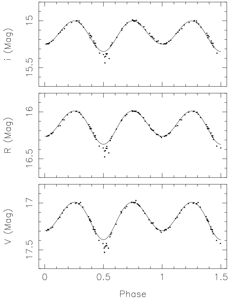
Fig. 2. V , R and i light curves of Nova Sco 1994 folded at the photometric ephemeris T_{\text{inf}}(\text{HJD}) = 244\,9838.4198(52) + 2.62168(14) \times N . The curves are repeated over 1.5 cycles for clarity. Phase 0.0 corresponds to inferior conjunction of the secondary with respect to the compact star. The drawn lines represent a theoretical light curve computed for a binary inclination and secondary mass of (67^\circ.25, 1.60 M_{\odot}) .
