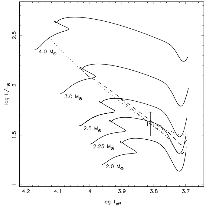
Fig. 10. Evolutionary tracks of single stars with mass 2.0 , 2.25 , 2.5 , 3.0 and 4.0 M_\odot (solid lines) and for stars in binary system which lose mass to their companion (dashed/dotted curves). The total system mass of the binary system is in all cases 9.2 M_\odot .
