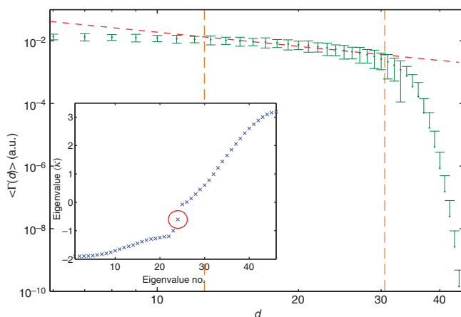
Figure 5 | Correlation with next-nearest-neighbour coupling. Shown is the simulation of the disorder-averaged correlation subjected to a next-nearest-neighbour coupling strength of 0.5\kappa . As before, 1,000 runs of 65 realizations have been simulated to allow a direct comparison with Fig. 3. The same length scales as in the experiment apply. The inset shows the eigenvalue spectrum, the gap state being highlighted by a red circle.
