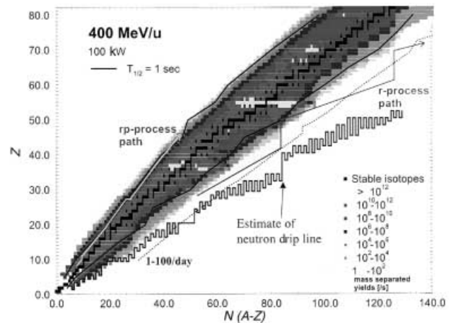
Figure 2: RIA yields from a multibeam driver; mass-separated intensities. (Courtesy ANL)
