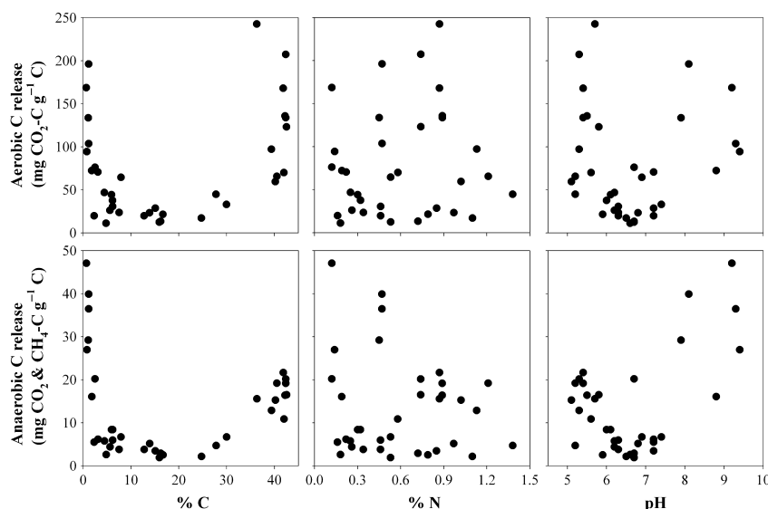
Fig. 5 The correlation among soil %C, %N and pH and cumulative C release per gram of soil C in permafrost soils after 500 days of incubation at 15\text{ }^\circ\text{C} under aerobic and anaerobic conditions.
