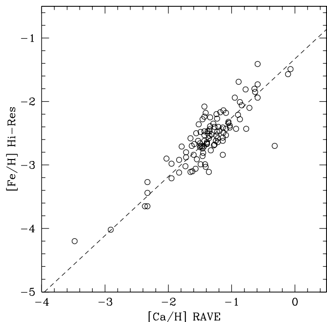
Figure 2. Calibration of the calcium abundance derived from the RAVE spectra onto iron abundance, using [\text{Fe}/\text{H}] from high-resolution echelle spectra, for 112 stars.
