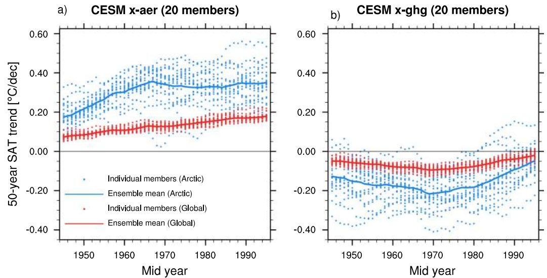
Figure 3. As in Figure 2c, but for (a) the 20 members of the Community Earth System Model v1 (CESM1) x-aer ensemble and (b) the 20 members of the CESM1 x-ghg ensemble.
