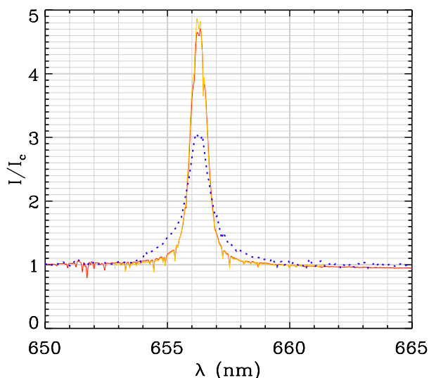
Fig. 2. Medium spectral resolution H \alpha CHARA/VEGA line profiles (blue dotted line) of \gamma Cas, recorded 2008 October 8. Red and yellow solid lines are amateur spectra obtained from the BeSS database, recorded on 2008 September 26 and October, 9.
