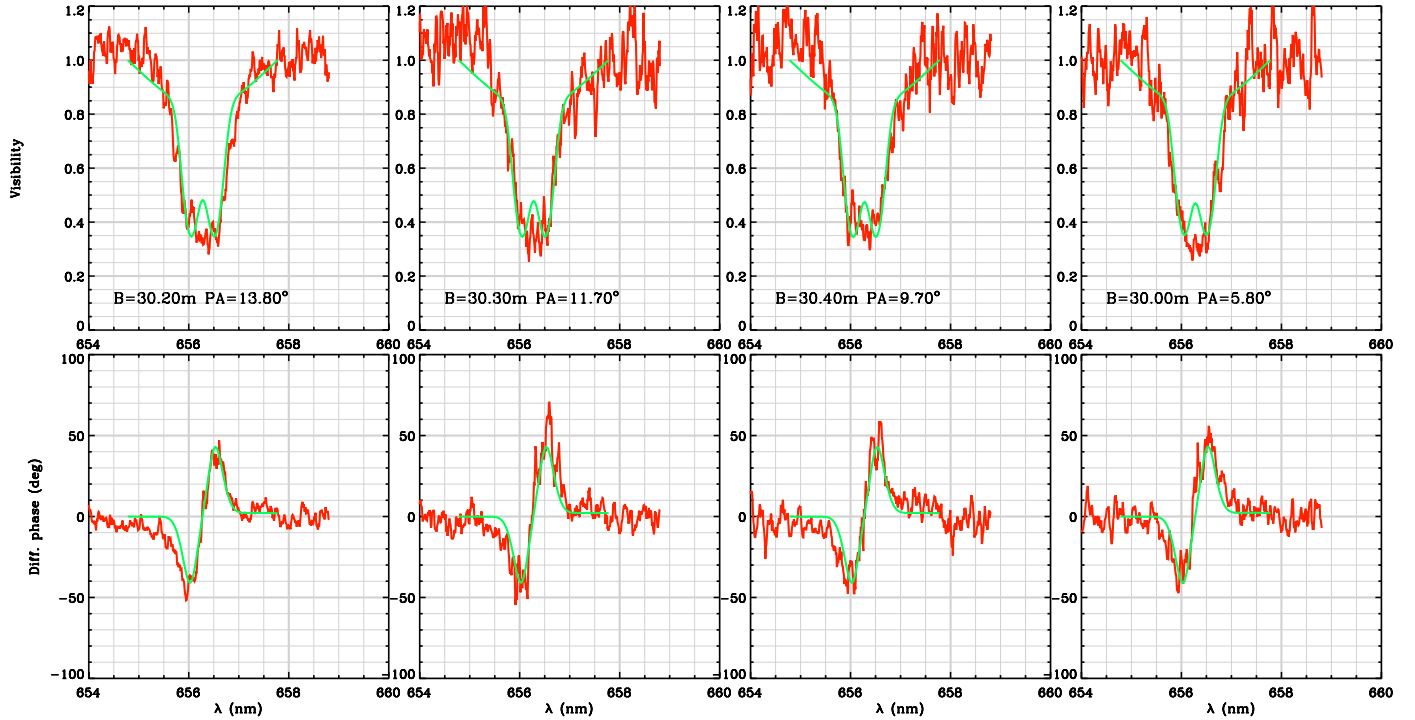
Fig. 8. \gamma Cas calibrated high spectral resolution (30 000) measurements: visibility ( top ) and differential phase ( bottom ) for different baseline lengths and PA indicated on each plot. The visibility and phase from our best-fit model is overplotted in green (plain line).
