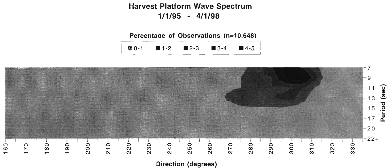
Figure 5. The Harvest Platform wave spectrum from January 1, 1995 to April 1, 1998 showing the relative percentage of observations for each direction and period used in the SCRDM model. The wave spectrum is characterized by 7–10 sec waves approaching from the northwest, particularly from the 291–309 deg range.
