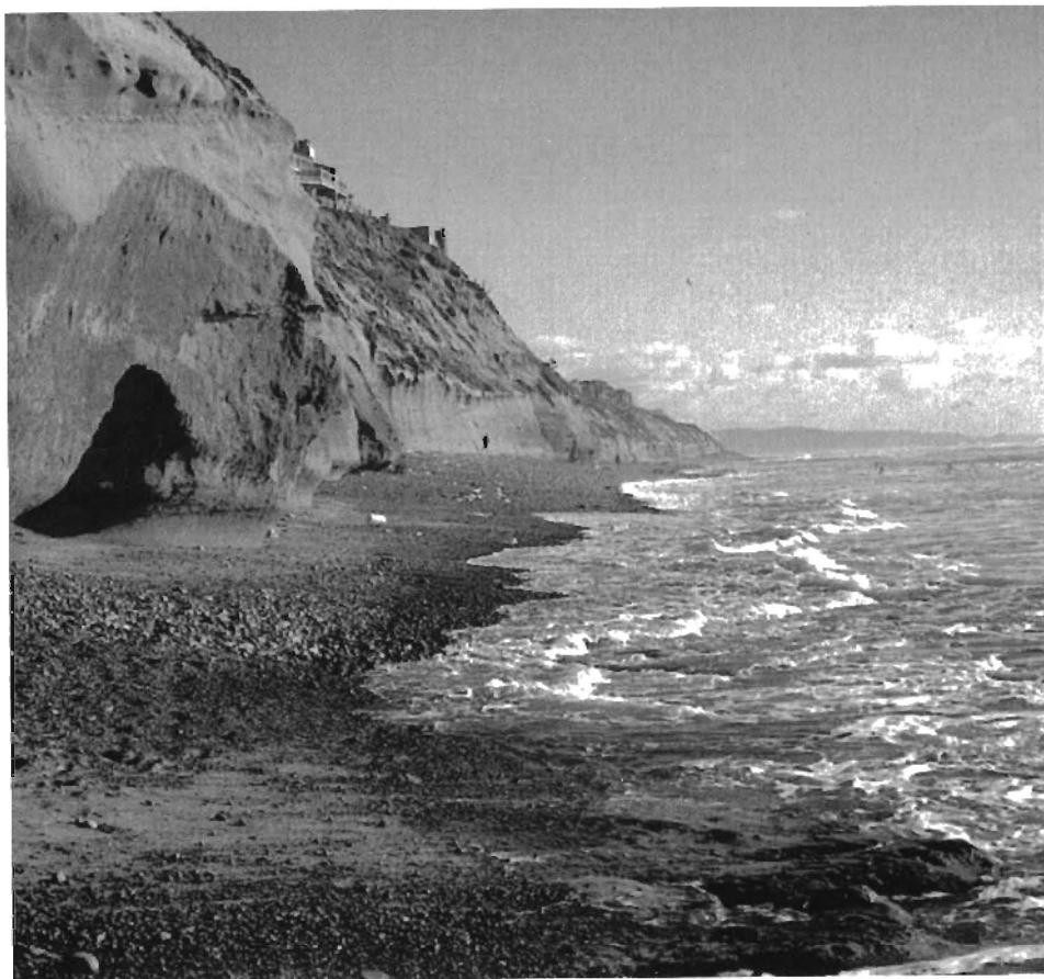
Figure 11. The Solana Beach site showing the landward extent of the low tide (0.3 m) wave (1–2 m) run-up. Wave-induced erosion of these cliffs is not limited to high tides.
