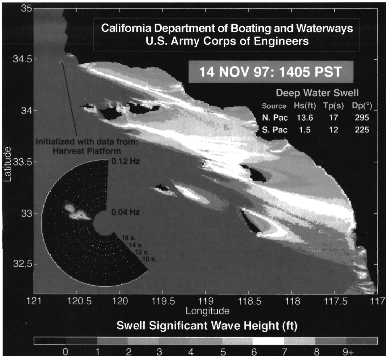
Figure 4. An example of the CDIP SRCDM wave model on November 14, 1997 showing the relative distribution of wave heights along the San Diego County coastline during a typical northwest swell. Note the lack of island sheltering along the La Jolla and Sunset Cliffs coastlines.
