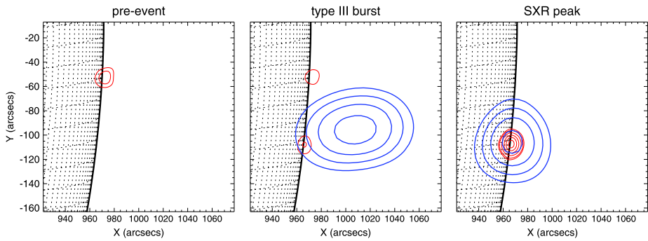
Fig. 15 RHESSI X-ray imaging before ( left ), during ( middle ), and after ( right ) radio Type III bursts. Thermal emission (4–8 keV) is shown in red contours (contours at 5, 10, 30, 50, 70, 90% of the level in the final panel ) with 10'' FWHM resolution, and the 14–30 keV emission is given in blue (levels are 65, 75, 85, and 95%) with a resolution of 60'' . From Krucker et al. (2008b)
