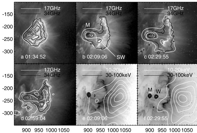
Fig. 9 The evolution of the radio and hard X-ray sources later in SOL2002-08-24T01:12 (X3.1). The first four images show a sequence of overlays of 17 GHz ( white contours ) and 34 GHz ( black contours ) images on TRACE 195 Å FeXII/FeXXIV images during the extended phase of the flare when the loop system is expanding above the west limb. The upper four contour levels are at 30, 50, 70 & 90% of the maximum in each image, while the lowest contours are at 10, 4, 2 & 1%, respectively, to match the changes in the peak intensity. RHESSI observes the early impulsive phase of the event and then goes into eclipse until 02:08 UT, and the last two images show contours of the RHESSI 10–20 keV ( white ) and 30–100 keV ( black ) emission overlaid on the TRACE 195 Å FeXII/FeXXIV images at 02:09:56 UT and 02:29:55 UT (displayed with inverted color table). The prominent nonthermal radio source is visible at the eastern base of the radio emission from 02:00 UT onwards. The radio emission from the loop tops at the northern end of the arcade has a flat spectrum and hence is probably thermal free-free emission. The 10–20 keV hard X-rays originate above the EUV loops, in higher soft X-ray emitting loops, while the harder 30–100 keV X-rays originate at the same location as the nonthermal radio source. From Kundu et al. (2004)
