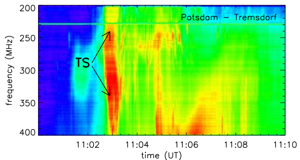
Fig. 16 The dynamic spectrum of SOL2003-10-28T11:10 (X17.2), from the Tremsdorf spectrograph operated by the Astrophysikalisches Institut Potsdam. The bright chevron-shaped feature centered at 11:03 UT (labelled “TS”) is identified as a termination-shock feature
