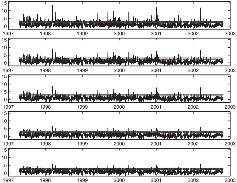
Figure 12 The five panels show observed values of the five daily jump statistics— z_{TP,t} , z_{TP,l,t} , z_{TP,lm,t} , z_{TP,r,t} , and z_{TP,ym,t} —computed using the five-minute returns on the S&P cash index, April 21, 1997–October 22, 2002. The horizontal lines are the upper 0.99 and 0.999 critical values of the standard Gaussian distribution.
