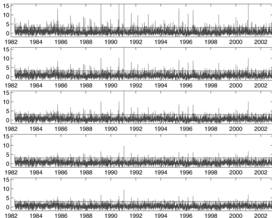
Figure 13 The five panels are the time series plots of the observed values of the daily statistics— z_{TP,t} , z_{TP,t,t} , z_{TP,lm,t} , z_{TP,r,t} , and z_{TP,rm,t} —computed using the five-minute returns on the S&P index futures, April 21, 1982–December 9, 2002. The horizontal lines are the upper 0.99 and 0.999 critical values of the standard Gaussian distribution.
