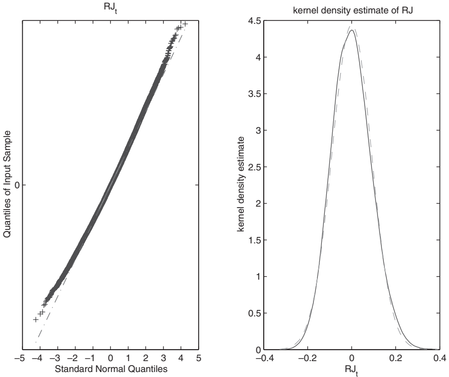
Figure 6 QQ plot and kernel density plot, RJ_t daily statistic for 45,000 days, using five-minute returns under medium mean reversion ( \alpha_v = -0.100 ).
