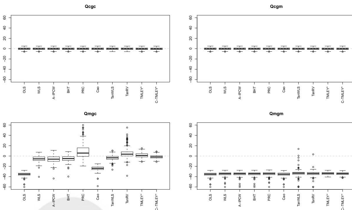
Figure 2: Sampling distribution of (\mu_n - \mu_0) with g_n bounded at 0.025, Modification 1 of Kang and Schafer simulation.
