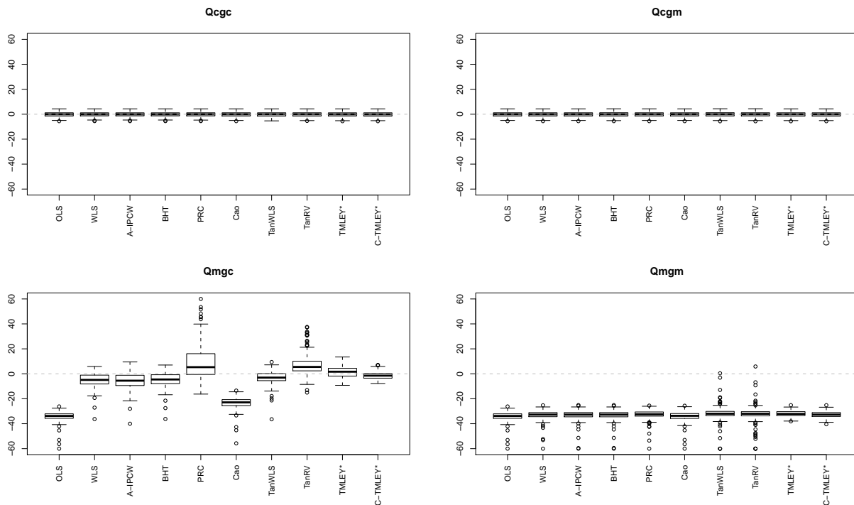
Figure 3: Sampling distribution of (\mu_n - \mu_0) with g_n bounded at 0.025, Modification 2 of Kang and Schafer simulation.
