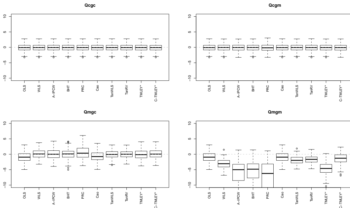
Figure 1: Sampling distribution of (\mu_n - \mu_0) with no bounding of g_n , Kang and Schafer simulation.
