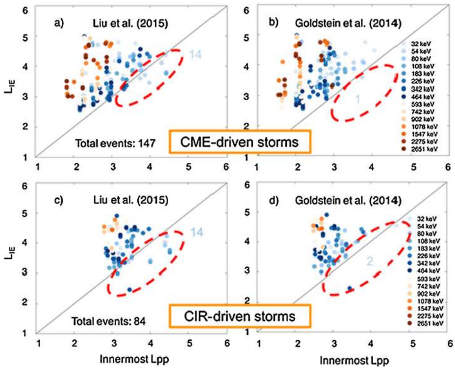
Fig. 19 Relationship between the innermost plasmopause location (as predicted by two distinct models) and the initial enhancement location of radiation belt electrons. The results show that nearly all enhancement events occurred outside the plasmopause in either plasmasphere model, and the enhancement location L_{IE} showed a distinct energy dependence. After Khoo et al. 2019
