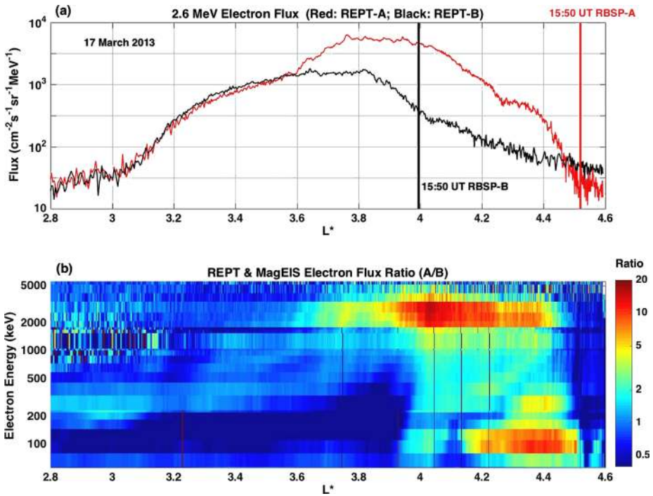
Fig. 26 (a) Sequential profiles of 2.6 MeV electron flux measured by the dual Van Allen Probes are shown. During the event, RBSP A followed RBSP B by \sim 1 h along the same orbital trajectory. RBSP B was at L^* \sim 4.0 at the 1550 UT substorm onset, while RBSP A was at L^* \sim 4.5 . On its inbound orbit RBSP B observed presubstorm background fluxes over L^* \sim 4.5 – 4.0 , while RBSP A observed postsubstorm enhancements. The plasmopause was observed at L^* \sim 2.5 at 1710 UT. (b) Ratios of electron flux (RBSP A (post substorm)/RBSP B (presubstorm)) are shown up to ultrarelativistic energies using MagEIS and REPT combined data (REPT data \geq 1.8 MeV). Injected \sim 50 – 150 keV electrons were seen at 31 RBSP A between L^* \sim 4.5 and 4.1 . The prompt onset of strong ( > 10x ) enhancements of \sim 1 – 3 MeV electron flux characterize the effects of local acceleration processes during the event
