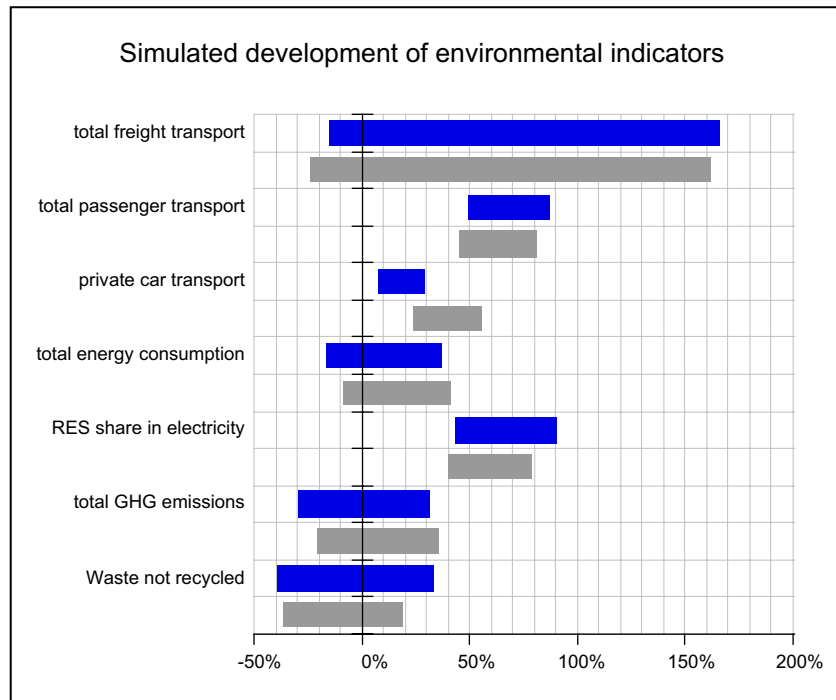
Fig. 3. Simulated development of environmental indicators by 2020 in % increase or decrease of their values in the base year 2000. The length of the bars indicates the uncertainty of the results that is caused both by future scenario variation and data uncertainty. There are two bars per indicator, the upper (dark) bar showing the results for the projected ICT development, the lower (light) bar showing the results for the so-called “ICT freeze” simulations (i.e. ICT applications remain at the level of 2000). Private car transport is included in total passenger transport, but also displayed separately to show the modal split in passenger transport. Abbreviations: RES = Renewable Energy Sources, GHG = GreenHouse Gas.
