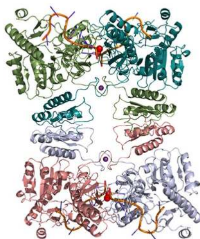
Figure 2 - Structure of RNase E in complex with RNA substrate. Crystal structure of the catalytic domain of E. coli RNase E, PDB ID 2C4R. RNA substrate in complex with the enzyme is coloured in orange and the metal ions that assist catalysis are shown as red spheres. Purple spheres denote the Zn 2+ ions important for maintenance of the principal dimers in the RNase E quaternary structure. Structure was drawn using PyMOL ( http://pymol.sourceforge.net ).
