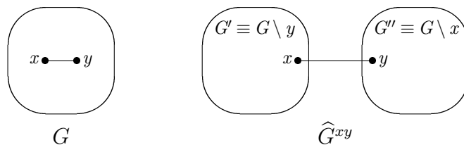
Figure 1: The graphs G and \widehat{G}^{xy} .
