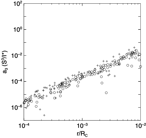
Fig. 4. Residual acceleration (radial component), as for Fig. 2, for the Poincaré dodecahedral space S^3/I^* .
