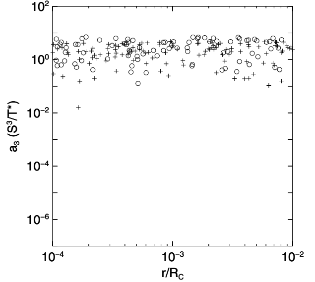
Fig. 2. Residual acceleration (radial component) induced on a test particle near a massive particle by the eight adjacent topological images of the massive particle, in a universe whose 3-manifold of comoving space is the octahedral space S^3/T^* . The accelerations a_3(r) are normalised to be constant if the dominant term is third order in r/L_q (see Eq. (19)) and are shown against distance r < 250 h^{-1} Mpc = 0.01R_C from the massive particle. Positive accelerations are shown by plus symbols; negative accelerations are shown by circles.
