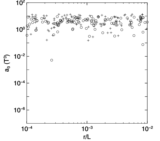
Fig. 1. Residual acceleration (radial component) induced on a test particle near a massive particle such as a cluster of galaxies by the six adjacent topological images of the massive particle, in a T^3 universe of three exactly comoving equal side lengths L_a . The accelerations a_3(r) are normalised to be constant if the dominant term is third order in r/L_a (see Eq. (14)) and are shown against distance r < 0.01L_a from the massive particle, where L = 3000 h^{-1} Mpc. Positive accelerations are shown by plus symbols; negative accelerations are shown by circles.
