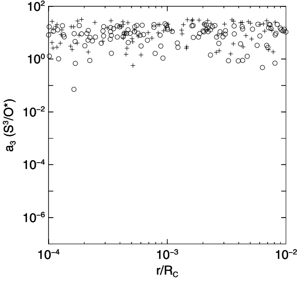
Fig. 3. As for Fig. 2, for the truncated cube space S^3/O^* .
