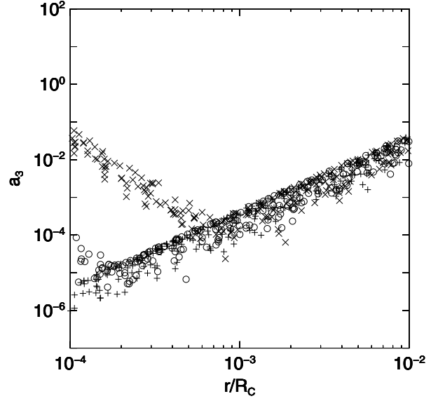
Fig. 5. Orthogonal residual acceleration for the Poincaré dodecahedral space S^3/I^* , as for Fig. 4, shown using 50-bit ( \times ), 60-bit ( \circ ) and 70-bit ( + ) precision in the significands of the floating-point numbers.
