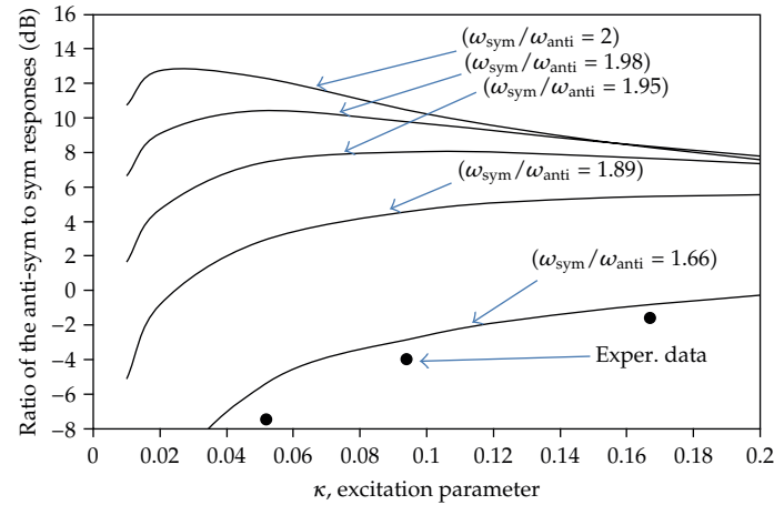
Figure 5: Ratio of the antisymmetrical to symmetrical responses, (dB scale).
