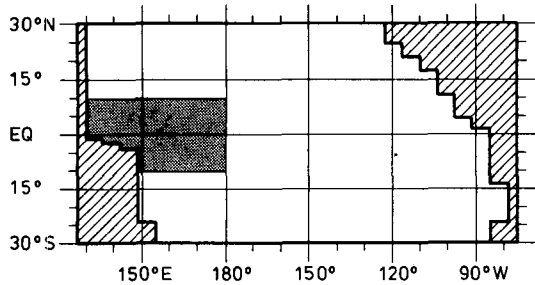
FIG. 1. Domain of the ocean model. The shaded area indicates the region of anomalous forcing.
