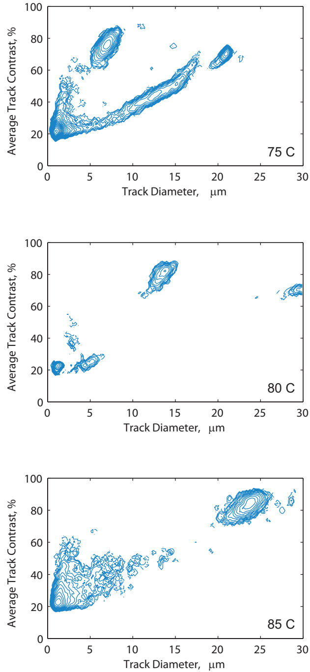
FIG. 9. Contours of constant number of tracks as a function of track contrast and diameter for a 6 hour etch at 75°C, 80°C and 85°C of 6 N NaOH. Two distinct islands of contours are visible in each plot: noise which occupies the bottom-left corner of contrast-diameter space and proton tracks which occupy the upper region and shift to the right for increasing etch temperatures.
