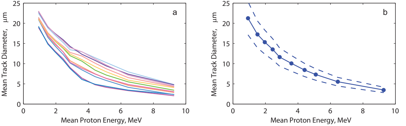
FIG. 2. (a) Proton track diameter as a function of incident mean energy for TasTrak CR-39 from 11 separate exposures; each piece was etched for 6 hours in an 80°C solution of 6 N NaOH. Variability in the shape of the curves from one piece to the next is observed. (b) Average (solid line) and standard deviation (dashed line) of proton track diameters as a function of incident mean energy computed using results from the 11 separate exposures of Fig 2a.
