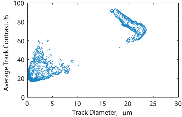
FIG. 7. Contours of constant number of tracks as a function of track contrast and diameter for DD-p fusion products ranged down to 920 keV. The proton tracks are in the top right corner of the plot with intrinsic noise occupying regions of lower contrast and smaller diameter. Note how the diameter distribution turns around for these protons, resulting in the non-gaussian diameter distribution of Fig. 1c.
