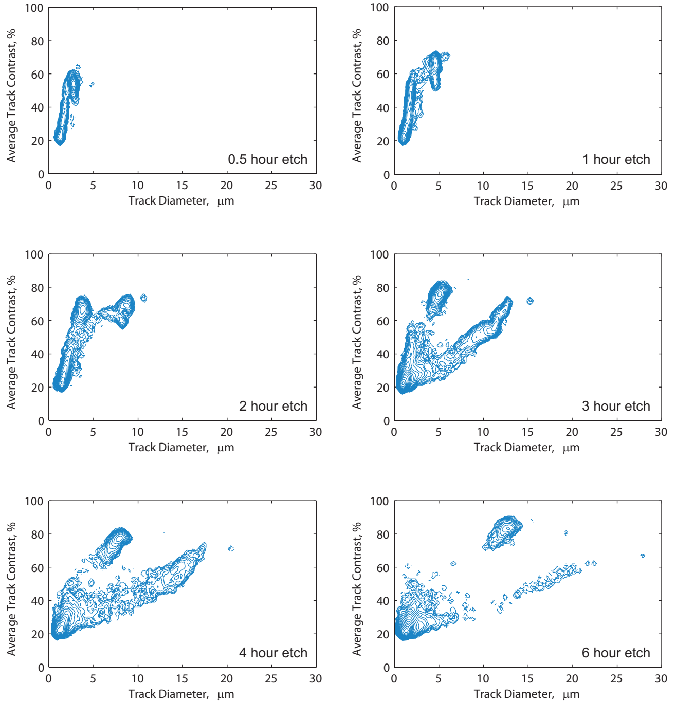
FIG. 8. Contours of constant number of proton tracks as a function of track contrast and diameter for a single piece of CR-39 etched in stages. Shown are data for 3.6 MeV protons generated by ranging down D- 3 He fusion protons with the use of aluminum filters. As the etch time is increased, the proton tracks shift towards higher contrast and larger diameters, making them more distinct from intrinsic noise.
