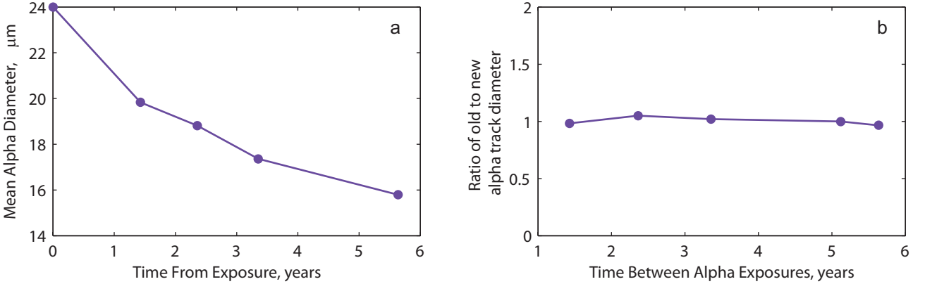
FIG. 6. (a) Track diameter of alpha particles as a function of time between exposure of CR-39 pieces to 5.5 MeV alphas and etching. Each of these pieces was kept at room temperature with minimal exposure to light for the time periods shown. (b) The effects of aging on alpha-track diameter are independent on the time of exposure. CR-39, which had been previously exposed to alpha particles, was exposed again to alpha particles just prior to etching. The differences between new and old track diameters are \sim 5\% .
