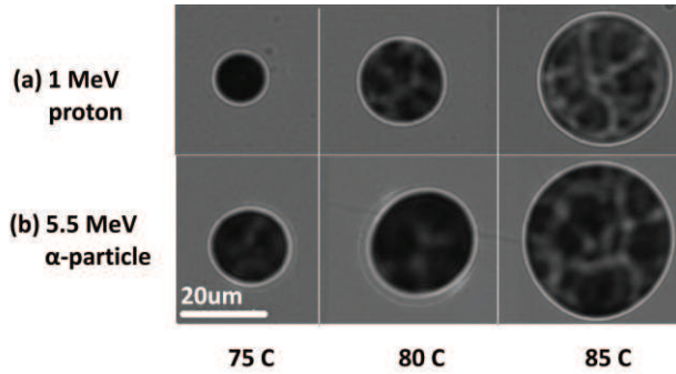
FIG. 5. Microscope images (at 40\times magnification) of (a) 1 MeV proton and (b) 5.5 MeV alpha particle tracks on CR-39, illustrating the non-uniformity of track contrast with increasing etchant temperature. Images were taken from three samples, each containing protons and alphas.
