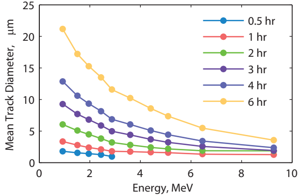
FIG. 3. Proton track diameters as a function of incident mean energy for various etch times. Four samples of CR-39 were stage-etched in steps from 30 minutes up to 6 hours in a 6 N NaOH solution at 80°C; the results between the four pieces have been averaged to eliminate any piece-to-piece variation. A linear response between etch time and track diameter is demonstrated. Note that for a 30 minute etch, protons with energies greater than 3 MeV are not detected and hence not shown.
