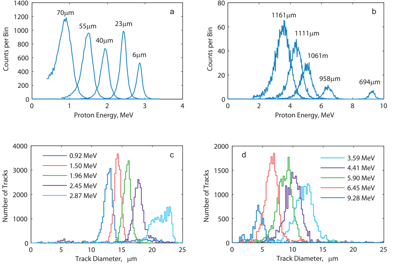
FIG. 1. Energy distribution function of protons used in this study. Protons were generated from 3 MeV DD or 14.7 MeV D^3He fusion products with the use of stepped aluminum filters, which were overlaid on the CR-39 sample; filter thicknesses are indicated above respective peaks. Energy distributions were measured with a detector system utilizing a 2000 \mu\text{m} thick silicon surface barrier detector (SBD); the energy accuracy of the system was \pm 75 keV.
