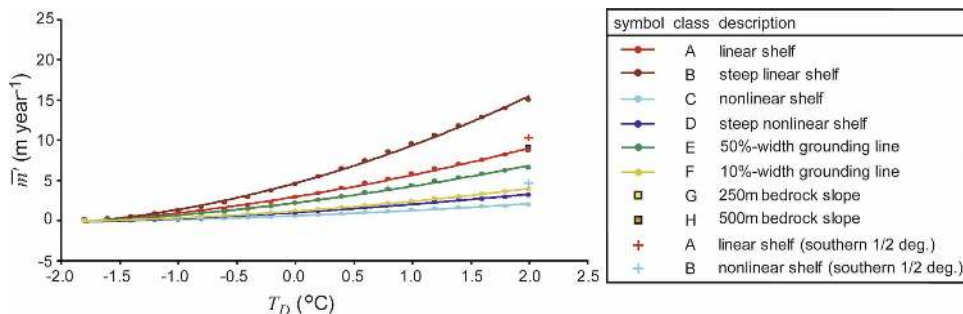
FIG. 7. The relation between mean melt rate and thermal forcing for all simulation classes used in this study. Curves drawn are quadratic fits to the results of classes A–F; the results of all classes exhibit quadratic behavior.
