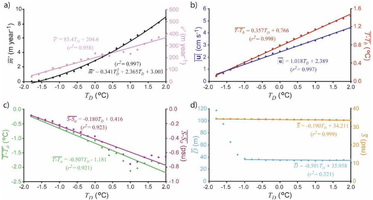
FIG. 5. The relations between mixed layer properties averaged over the area beneath the ice shelf and thermal forcing from all simulations in class A: (a) ice shelf melt rate and mixed layer entrainment rate, (b) mixed layer speed and mixed layer–interface temperature difference, (c) temperature and salinity differences between the mixed layer and its entrained water, and (d) mixed layer thickness and salinity.
