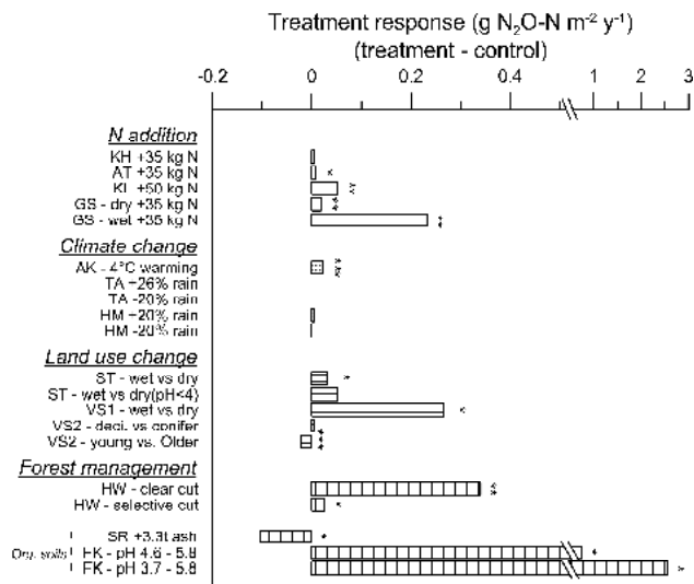
Fig. 2. Response of N 2 O gas exchange to forest change (treatment minus control). Site codes and treatments are explained in Table 1. Stars indicate the level of significance for the treatment effect (*: p < 0.05 ; **: p < 0.01 ; ***: p < 0.001 ).
