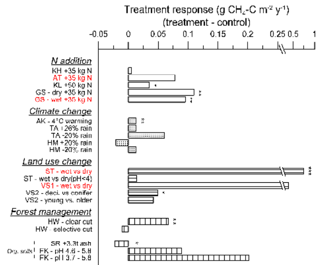
Fig. 3. Response of CH 4 gas exchange to forest change (treatment minus control). Site codes and treatments are explained in Table 1. Stars indicate the level of significance for the treatment effect (*: p < 0.05 ; **: p < 0.01 ; ***: p < 0.001 ). A positive treatment response indicates that more CH 4 is left in the atmosphere (i.e. a lower CH 4 uptake occurred in the treatments compared to the controls). The text in red marks the sites that had CH 4 emission (AT) or where the treatment resulted in a net CH 4 emission (GS-wet, ST and VS1).
