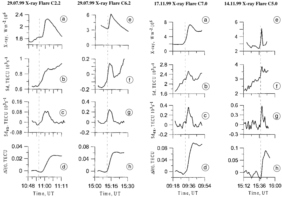
Fig. 2a-h. Faint solar flare July 29, 1999 (C2.2, 11:00 UT) (a-d); soft X-ray emission flux (GOES-10) in the range 1-8 Å (a); normalized result of a coherent summation Sd of the time derivatives of the TEC variations for all LOS (b); the same curve (b), upon subtracting the trend determined as a polynomial of degree 3 on the time interval 10:48-11:11 UT; mean integral increment of TEC (d). Analogous dependencies for faint solar flare July 29, 1999 (C6.2/SN, 15:14 UT, N25E53) on panels (e-h).
