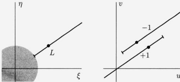
FIG. 3. Wave curves for s = \pm 1 . For clarity's sake, we show wave curves through different states with the same (\xi, \eta) components but slightly different (u, v) components.
