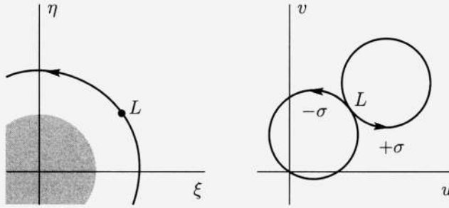
FIG. 2. Wave curves for s = \pm\sigma .
