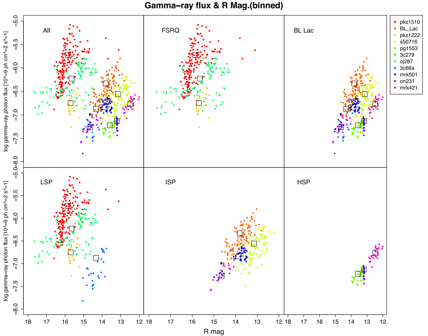
Figure 3. The sample plots as Fig. 2 with optical data points binned according to the range of the Fermi bins. There are fewer data but the overall trends are similar.
