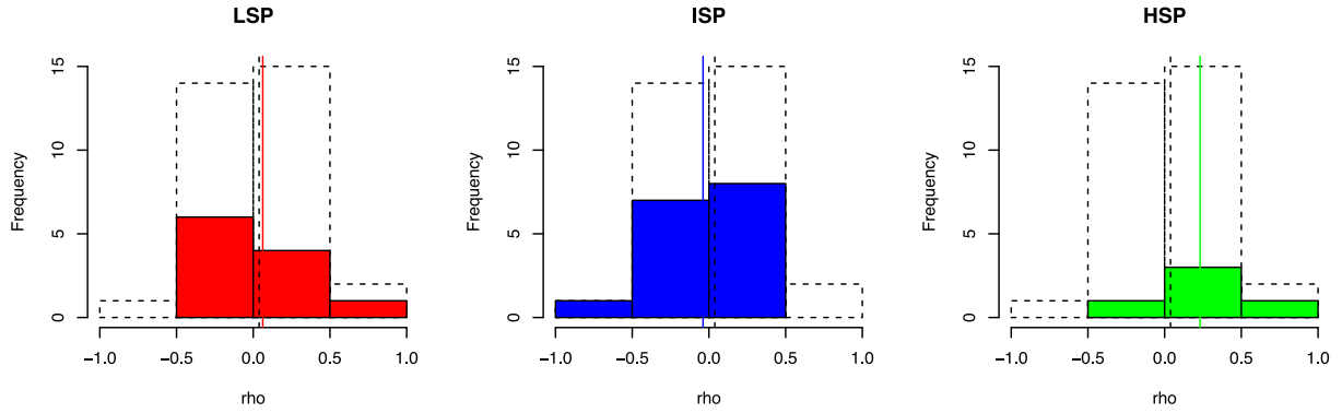
Figure 5. Histograms showing the distribution of \rho values from the Spearman Rank Coefficient test for the optical degree of polarization and \gamma -ray flux. From left to right: LSPs (red), ISPs (blue) and HSPs (green). The dotted histograms are the distribution of the total sample and the black vertical lines show where the sample mean lies. The mean of the subclasses are shown as a vertical line in their respective colours.
