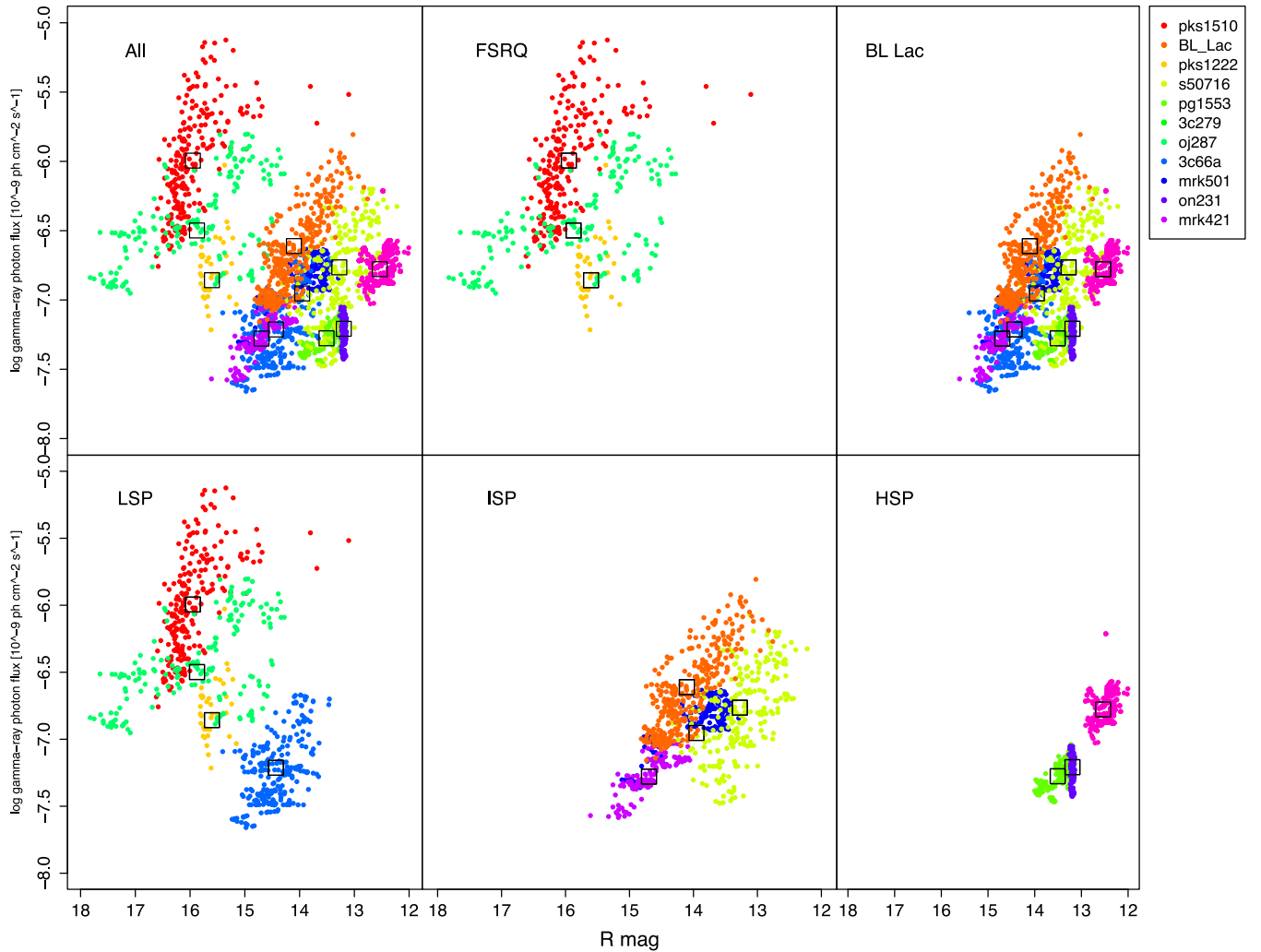
Figure 2. Fermi \gamma -ray data plotted against magnitude for 11/15 sources (those which have >5 \gamma -ray data points) (each with a separate colour) and subsequent blazar subclasses: FSRQs, BL Lacs, LSPs, ISPs and HSPs. The \gamma -ray data points are interpolated to match the date of the optical data points (see Section 4.1). Black squares show the mean \gamma -ray and optical value for each source.
