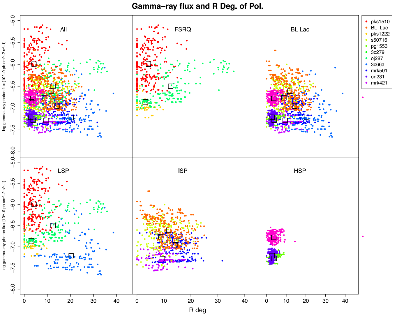
Figure 4. Fermi \gamma -ray flux against optical degree of polarization for all sources and each blazar subclass, a different colour for each source separately. Black squares show where the mean of the source lies on the plot. Horizontal and vertical lines in the data show periods during which the \gamma -ray/optical data (respectively) are constant while the other continues to vary.
