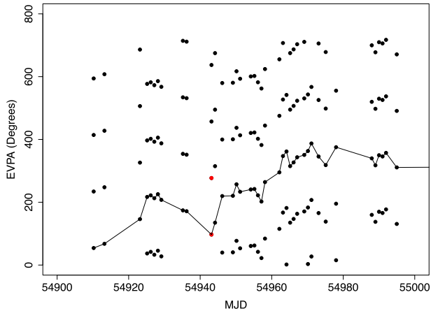
Figure 1. Zoomed view of PKS 1510-089 light curve (full light curve shown in appendix, Fig. A2). This plot can be compared with fig. 4 in Marscher et al. (2010) where the polarization angle data are interpreted as showing a 720^\circ rotation. Here we report a rotation of less than half that ( 333^\circ ) and this is due to the interpretation of this particular data set by the EVPA trace code which, to account for the \pm 180 , ambiguity identifies the next nearest lying point. The points in red highlight where the difference in identification originates.
