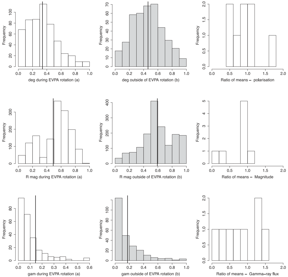
Figure 8. The degree of polarization (top), optical magnitude (middle) and \gamma -ray flux (bottom) displayed as a fraction of the normalized range for (a) during EVPA rotations (white) and (b) outside of EVPA rotations (grey) and (c) as a ratio of the mean of each property during a rotation over the mean of each property outside of a rotation for each individual source (see Section 4.2 for more details). The black vertical lines in the first two columns show the mean of the histograms.
