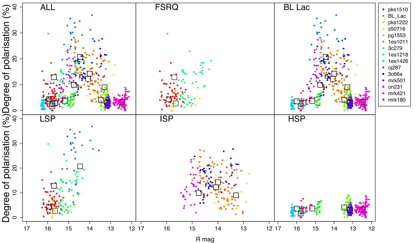
Figure 6. The optical degree of polarization against optical magnitude for all 15 sources. For those sources that do not have synchronous points (i.e. Mrk 421 and PKS 1222) we interpolate the nearest lying point from the neighbouring data points. Each source is coloured separately and black boxes show where the mean of that source lies on the plot.
