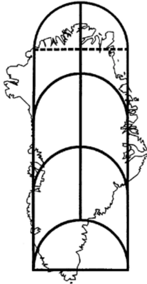
Figure 10. Schematic of bindschadler (1985) model. Extrapolating the 2-D model to three dimensions by a scaling factor of 5000 km is equivalent to assuming two parabolic cylinders back-to-back, with transverse (longitudinal) length of 2500 cm. Greenland is drawn to the same scale.
