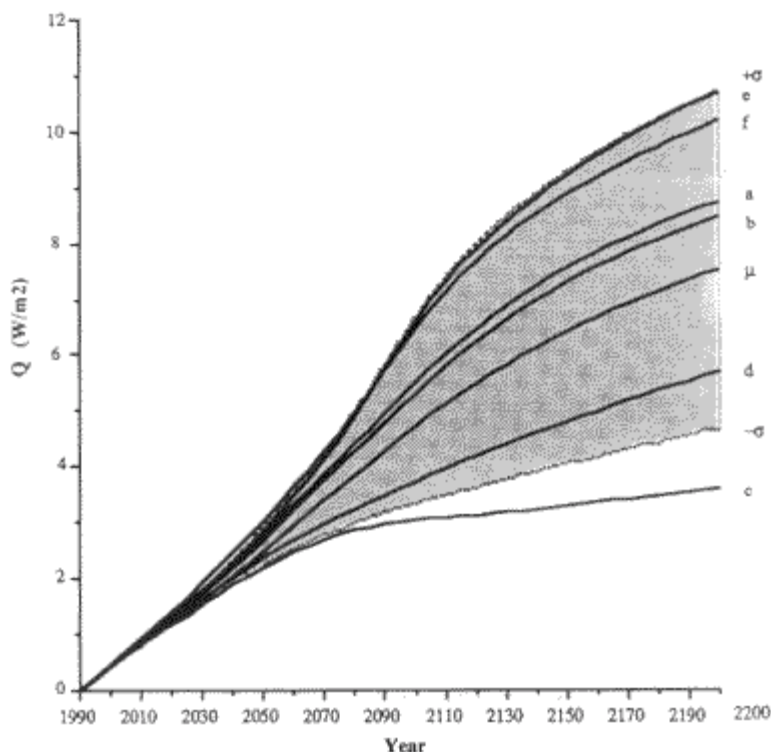
Figure 2. Comparison of greenhouse forcing probability distribution with forcing implied by IPCC (1992) emission scenarios. The shaded region shows the \sigma -limits for our analysis; \mu represents our median. The curves representing IPCC scenarios IS92a....IS92f were calculated using models and assumptions reported by Wigley and Raper (1992), except that emissions are assumed to be constant after the year 2100.
