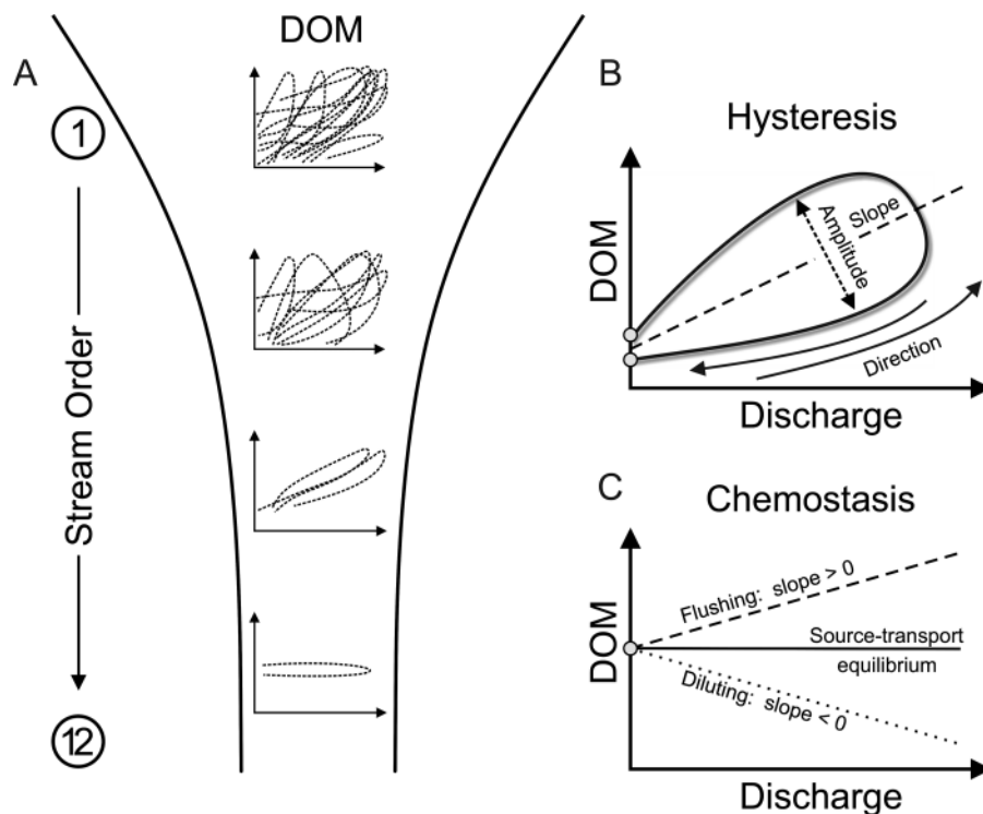
Fig. 5. Stream DOM reflects the nature of coupled terrestrial–aquatic water transport between terrestrial DOM source areas and the stream. (A) Low-order streams exhibit a range of hysteresis behaviours that converge toward chemostatic behaviour as river order increases. (B) The steeper the slope of the hysteresis loop (solid line), the higher the DOM gradient between terrestrial DOM source areas and the stream. A clockwise direction of change over the course of the event indicates that DOM sources are spatially connected to each other and proximal to the stream; a counterclockwise direction indicates DOM sources are spatially disconnected from each other and distal from the stream. The greater the loop amplitude, the greater the hydrological expansion into new terrestrial DOM sources. (C) Chemostasis occurs when DOM remains unchanged despite changes in discharge.
