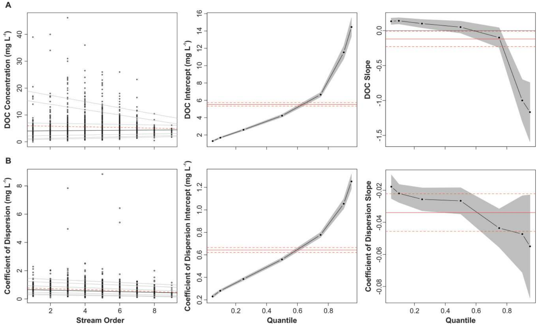
Fig. 3. Quantile regression analysis of (A) median DOC ( \text{mg}\cdot\text{L}^{-1} ) and (B) coefficient of dispersion of DOC ( \text{mg}\cdot\text{L}^{-1} ) as a function of stream order ( n = 1429 ). (Left column) The 95th, 90th, 75th, 50th, 25th, 10th, and 5th percentiles as a function of stream order (solid gray lines), the median fit regression (solid black line), and the least squares regression (red dashed line). Sample estimates of (middle column) intercept and (right column) slope of the relationship for each percentile, including endpoints of 90% confidence intervals (gray-filled area), the least squares regression estimate of the mean (solid red line), and the standard error of the mean (dashed red lines), are shown. Note that the quantile regression analyses are consistent whether the entire available dataset is used ( N = 1429 ) or the subset dataset for which \text{SUVA}_{254} exist ( n = 200 ). For the coloured version of this figure, refer to the Web site at http://www.nrcresearchpress.com/doi/full/10.1139/cjfas-2014-0400 .
