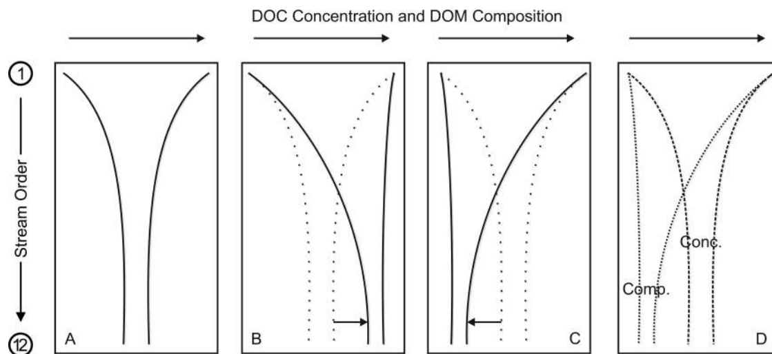
Fig. 8. A convergence of DOM variability to a downstream endpoint of chemostasis may reflect the relative influence of hydrological and biogeochemical processes. Three potential scenarios are as follows: (A) mixing waters from lower stream orders in equal proportions and instream production balanced by instream degradation; (B) greater relative contribution of high concentration DOC from lower stream orders and (or) instream net production of DOM; and (C) greater relative contribution of low concentration DOM from lower stream orders and (or) instream net degradation of DOM. Based on the first scenario in panel A, it is possible there is a change in DOM composition in large rivers despite no change in bulk DOC concentration (D).
