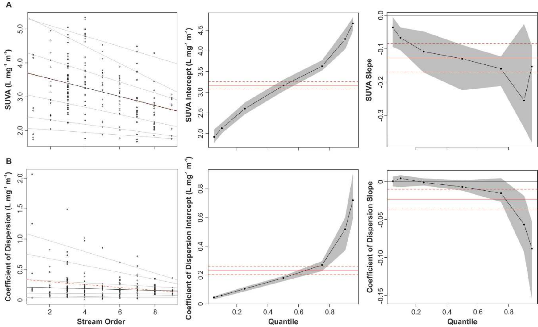
Fig. 4. Quantile regression analysis of (A) median SUVA_{254} ( L \cdot mg^{-1} \cdot m^{-1} ) and (B) coefficient of dispersion of SUVA_{254} ( L \cdot mg^{-1} \cdot m^{-1} ) as a function of stream order ( n = 200 ). (Left column) The 95th, 90th, 75th, 50th, 25th, 10th, and 5th percentiles as a function of stream order (solid gray lines), the median fit regression (solid black line), and the least squares regression (red dashed line). Sample estimates of (middle column) intercept and (right column) slope of the relationship for each percentile, including endpoints of 90% confidence intervals (gray-filled area), the least squares regression estimate of the mean (solid red line), and the standard error of the mean (dashed red lines), are shown. For the coloured version of this figure, refer to the Web site at http://www.nrcresearchpress.com/doi/full/10.1139/cjfas-2014-0400 .
