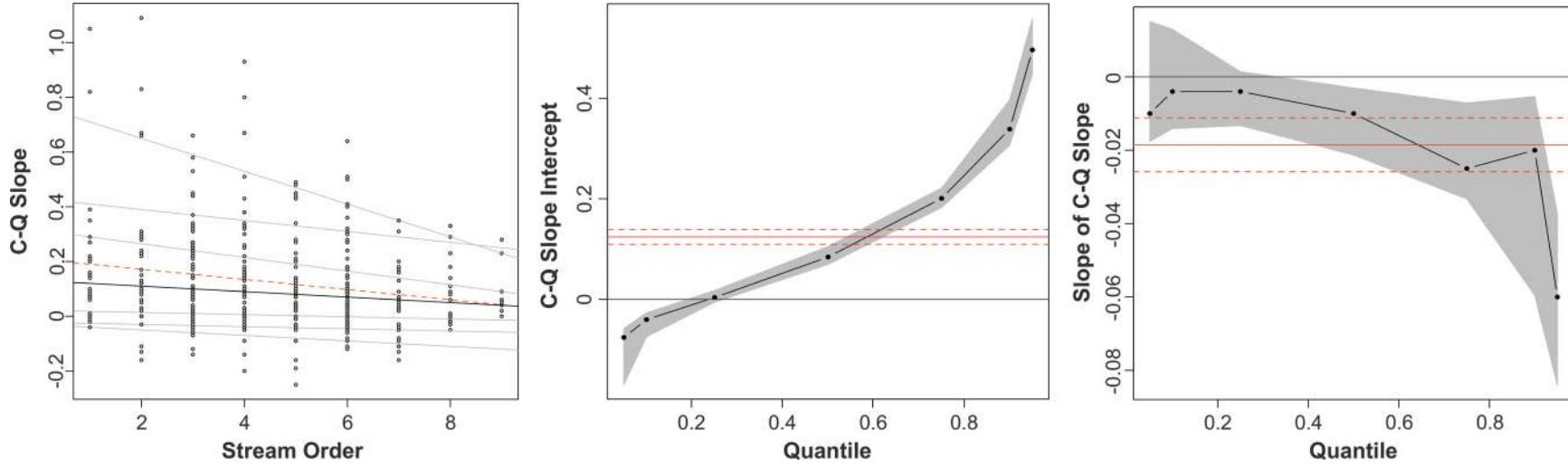
Fig. 6. Quantile regression analysis of median C-Q slope as a function of stream order ( n = 314 ). (Left column) The 95th, 90th, 75th, 50th, 25th, 10th, and 5th percentiles as a function of stream order (solid gray lines), the median fit regression (solid black line), and the least squares regression (red dashed line). Sample estimates of (middle column) intercept and (right column) slope of the relationship for each percentile, including endpoints of 90% confidence intervals (gray-filled area), the least squares regression estimate of the mean (solid red line), and the standard error of the mean (dashed red lines), are shown. Statistical analyses associated with quantile regression were not possible since there was insufficient C-Q slope data for each bin of stream order tested but indicated a linear, negative relationship for C-Q slope as a function of stream order for all percentiles (95th, 90th, 75th, 50th, 25th, 10th, and 5th). Statistical analyses associated with quantile regression were not possible since there were insufficient C-Q slope data for each bin of stream order tested. For the coloured version of this figure, refer to the Web site at http://www.nrcresearchpress.com/doi/full/10.1139/cjfas-2014-0400 .
