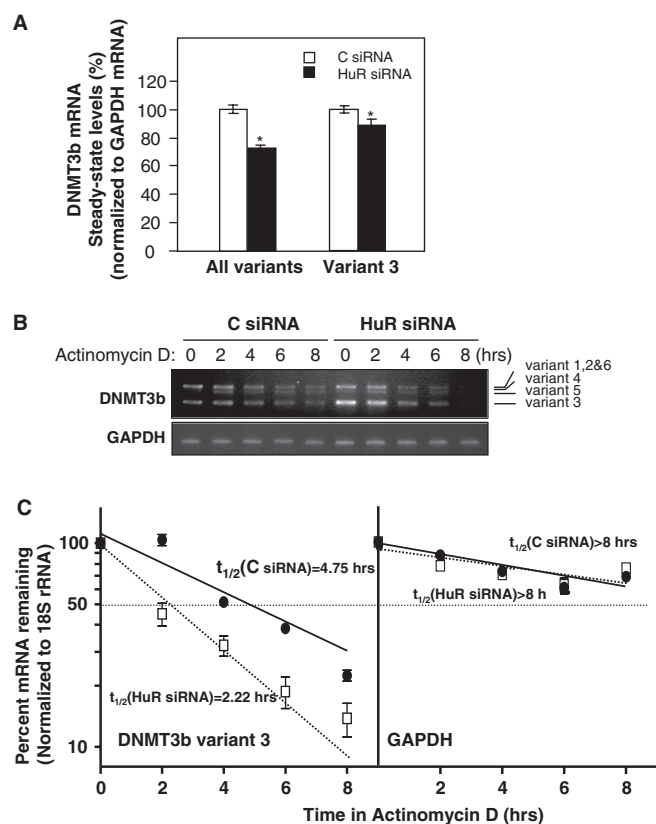
Figure 3. HuR silencing reduces DNMT3b mRNA stability and mRNA levels. (A) Two days after siRNA transfection, RKO cells were harvested, and RNA was analyzed by RT-qPCR (shown as the mean \pm SEM from three experiments; * P \leq 0.05 ). (B) The DNMT3b mRNA stability after silencing HuR was studied by incubating cells with actinomycin D, extracting total RNA at the times shown, and measuring DNMT3b mRNA levels by RT-PCR. Representative PCR products of all DNMT3b variants visualized in ethidium bromide-stained agarose gels are shown; the levels of GAPDH served to verify equal sample input. (C) DNMT3b variant 3 mRNA levels were measured by RT-qPCR. The data were normalized to 18S (house-keeping) mRNA levels and represented as a percentage of the mRNA levels measured at time 0, before adding actinomycin D, using a semi-logarithmic scale. The half-lives (indicated) were calculated as the time required for DNMT3b variant 3 mRNA decrease to 50% of its initial abundance (discontinuous horizontal line). Data represent the mean \pm SEM from three independent experiments.
