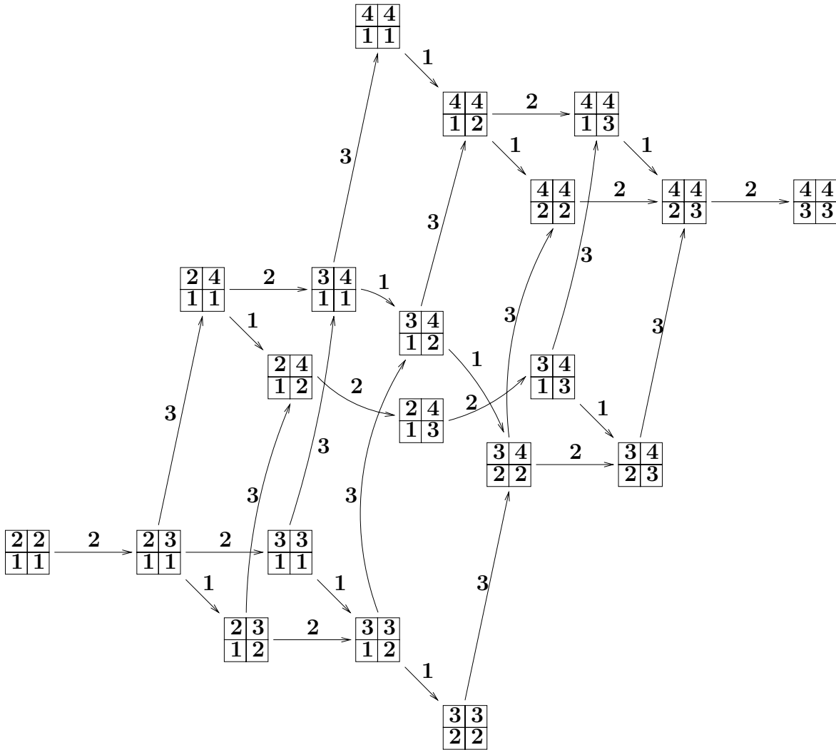
Figure 2: Crystal graph of the U_q(\mathfrak{gl}_4) -module V_{(2,2)}
