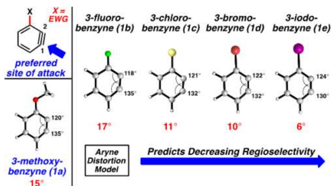
Figure 2. Geometry-optimized structures of 1a–1e (B3LYP) and regioselectivity predictions for nucleophilic attack based on the aryne distortion model.
