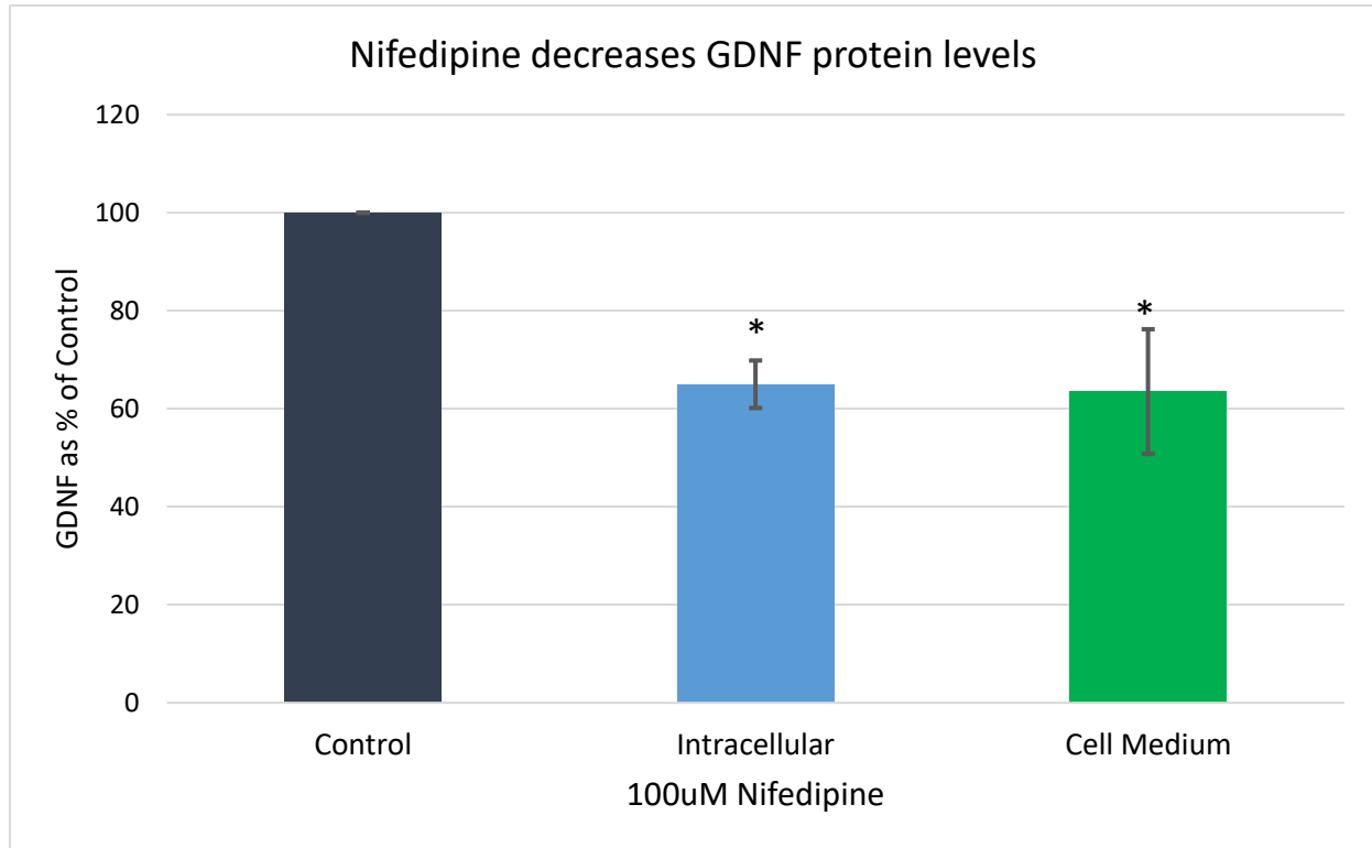
Figure 3: Effect of nifedipine on GDNF protein levels. C2C12 myotubes were treated with nifedipine ( 100\mu\text{M} ) and GDNF was measured with ELISA. Results show that the intracellular GDNF protein levels were decreased to 65.0% of control ( n=16 ). Extracellular GDNF protein levels were decreased to 63.5% of control myotubes ( n=8 ). The values shown here indicate the sample mean \pm SEM. The * indicates significance of p < 0.05 .
