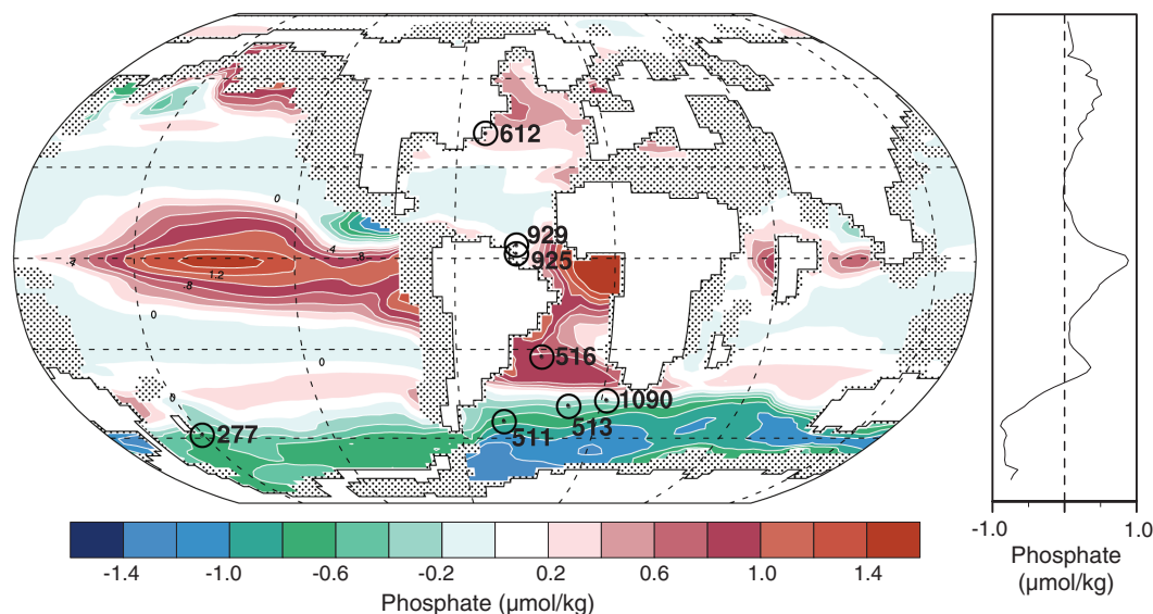
Fig. 1. DSDP and ODP sites used in this study overlain on model-derived surface ocean phosphate concentration anomaly. Sites are rotated back to their late Eocene paleo-positions. (Left) Contours indicate anomalies of the UVic climate-ecosystem-carbon cycle model-predicted surface ocean phosphate concentration (late Eocene simulation minus modern simulation; SOM). Modern continents are indicated by stippling, and Eocene continents are white with black outline. (Right) Zonal mean phosphate anomalies. Late Eocene continental configuration is associated with greatly reduced Southern Ocean phosphate and increased tropical and Northern Hemisphere phosphate.
