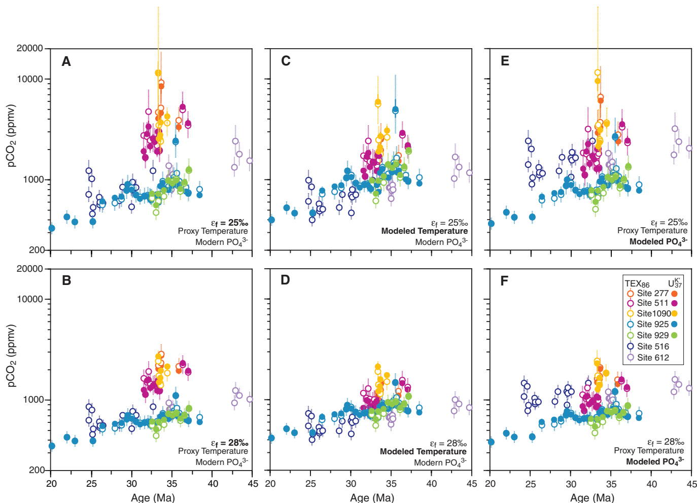
Fig. 3. Calculated p\text{CO}_2 from \epsilon_{\text{p37:2}} values. Error bars associated with each point reflect the uncertainty in \text{CO}_2 because of the temperature uncertainties for each temperature proxy. (A) p\text{CO}_2 calculated by using U_{37}^K and \text{TEX}_{86} values, assuming \epsilon_f = 25\text{‰} and using modern [\text{PO}_4^{3-}] averaged between 30 and 50 m for each paleolocation (SOM). (B) Same as (A) but using an
