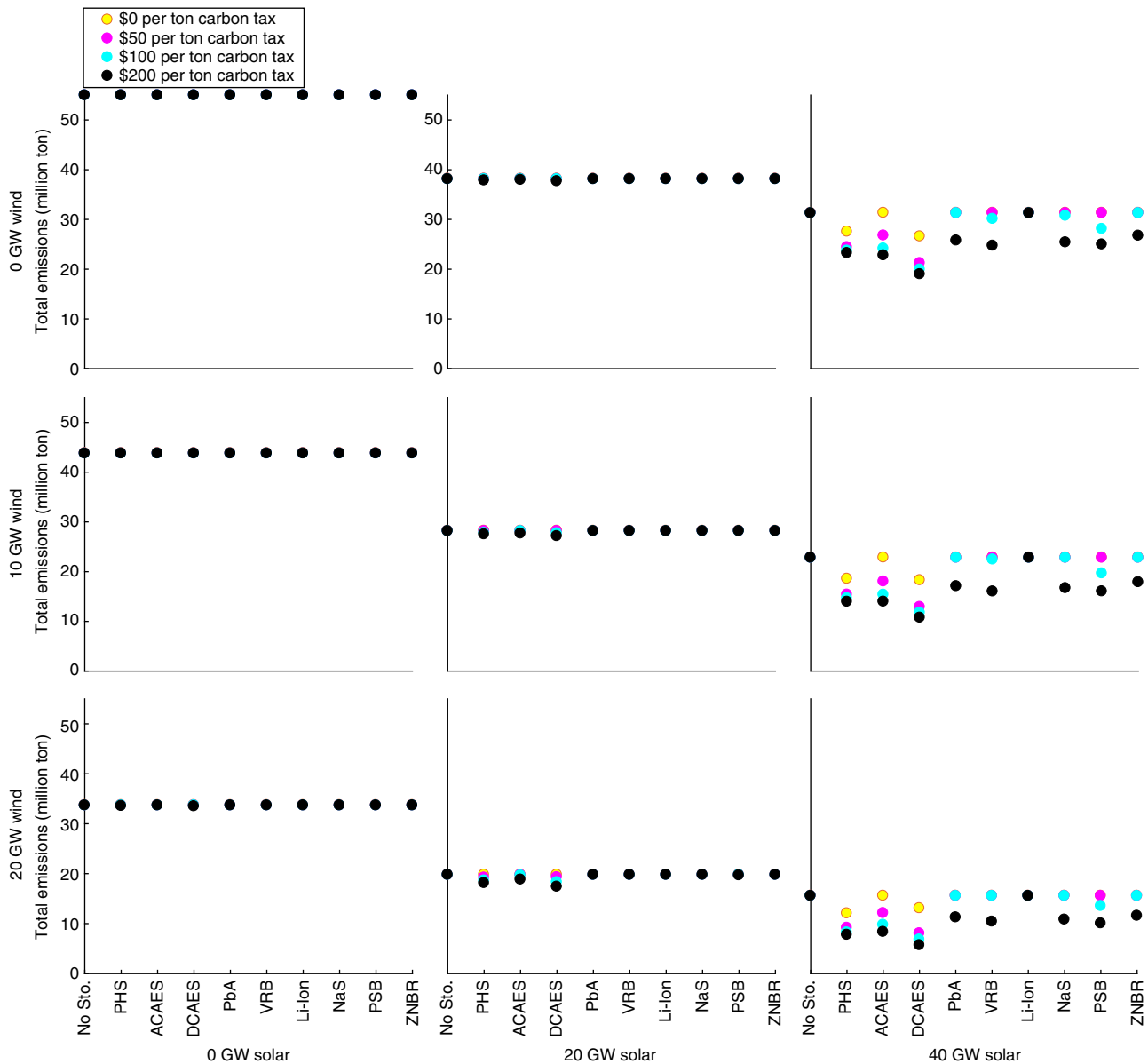
Fig. 3 Annual CO 2 emissions (million ton) in California for the year 2012 in the base case with a 7.0-GW minimum-dispatchability requirement. Figure panels correspond to different wind- and solar-penetration levels, which are indicated at the left-hand side and bottom, respectively, of the figure. Source data are provided as a Source Data file
