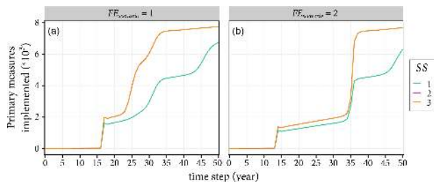
Figure 10. Impacts of subsidy on the adaptation behaviour of agents. The subsidy levers 1, 2 and 3 represent no subsidy, subsidy only for flooded household agents and subsidy for all agents that consider floods to be a threat, respectively. Panels (a) and (b) show simulation results with flood events scenarios of 1 and 2, respectively.
