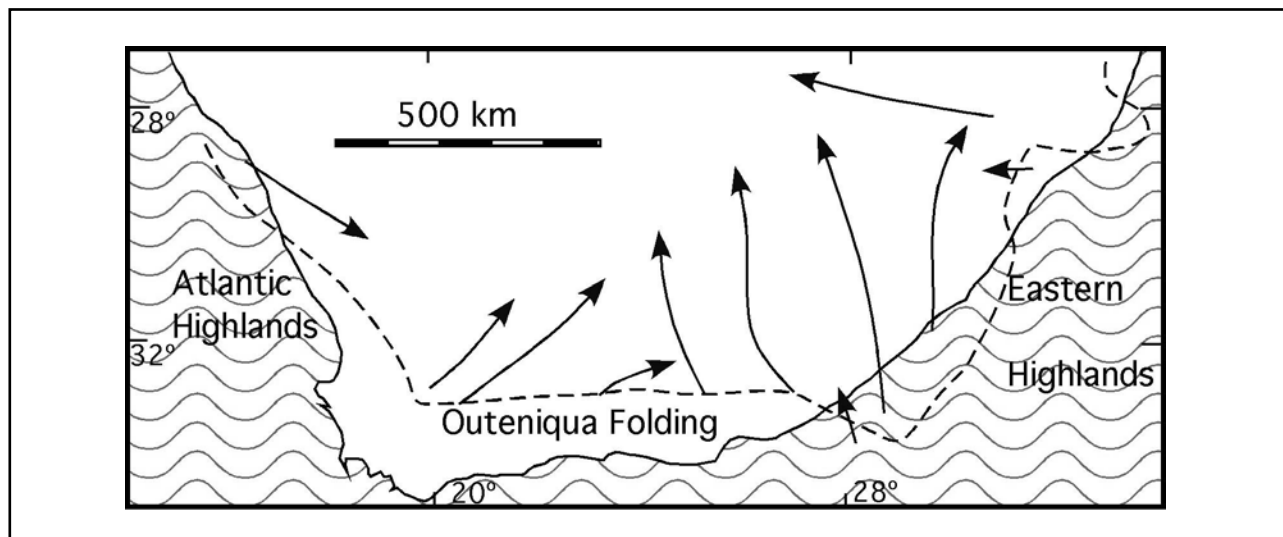
Figure 4. Late Permian – early Triassic (Beaufort Group) sediment dispersion patterns in southern Africa (after Veevers, et al. , 1994). This broad pattern persisted to the deposition of the late Triassic Elliot formation of the Stormberg Group, which is separated from the Drakensberg volcanics by the aeolian Clarens Formation.
