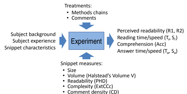
Fig. 2. Overview over all variables considered in the experiment.
