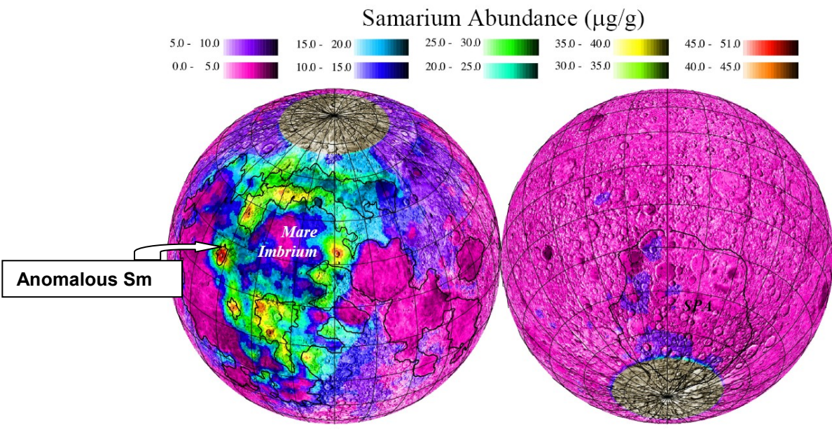
Figure 6 - Inferred Samarium Concentrations in the Imbrium/Procellarum Regions. From Elphic, et al. , 2000.
