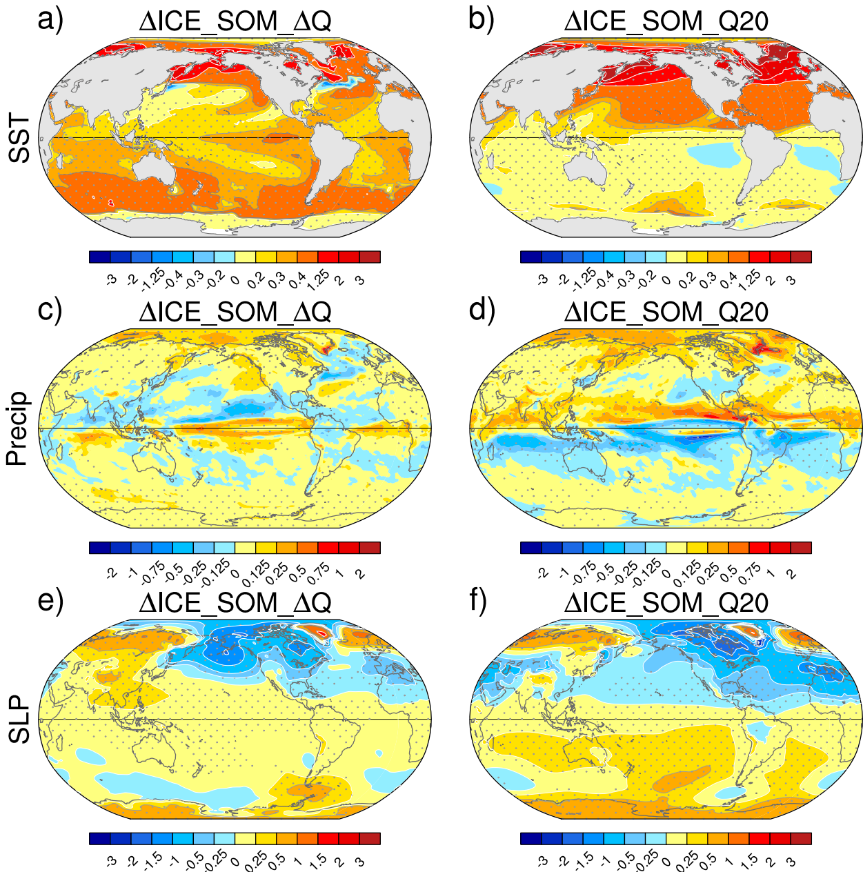
FIG. 4. As in Fig. 2, but for (left) \Delta\text{ICE\_SOM\_}\Delta\text{Q} .
