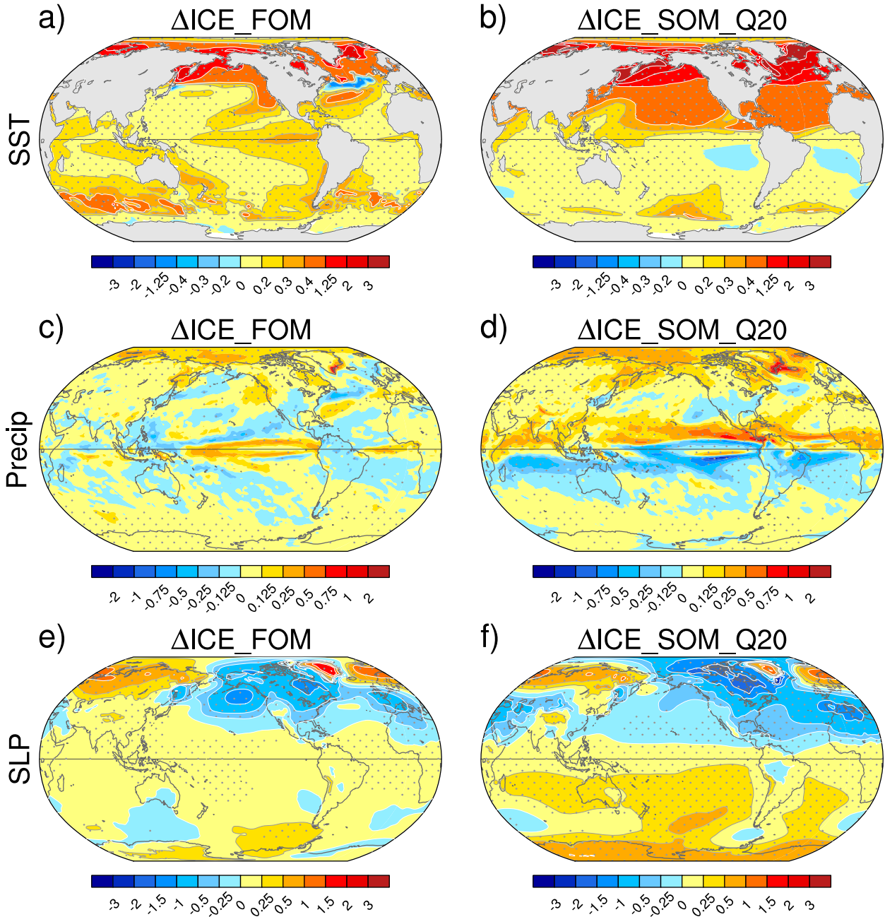
FIG. 2. Annual (a),(b) SST ( ^{\circ}\text{C} ), (c),(d) precipitation ( \text{mm day}^{-1} ), and (e),(f) SLP (hPa) responses to Arctic sea ice loss in (left) \Delta ICE\_FOM and (right) \Delta ICE\_SOM\_Q20 . Stippling indicates that the response is statistically significant at the 95% confidence level.
