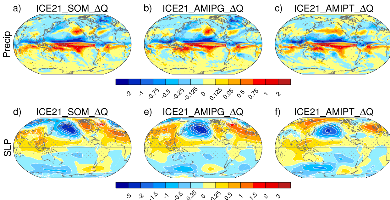
FIG. 11. December–February (a)–(c) precipitation ( \text{mm day}^{-1} ) and (d)–(f) SLP (hPa) responses in (left) ICE21_SOM_ΔQ, (center) ICE21_AMIPG_ΔQ, and (right) ICE21_AMIPT_ΔQ.
