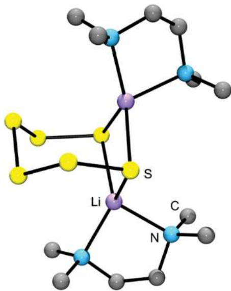
Fig. 6 Solid-state structure of [\text{Li}(\text{TMEDA})_2][\text{S}_6]^- determined by X-ray crystallography (bond lengths: \text{Li}-\text{S} 249 pm, \text{S}-\text{S} : 204–208 pm; adapted from Tatsumi et al. 1990, ref. 41).
